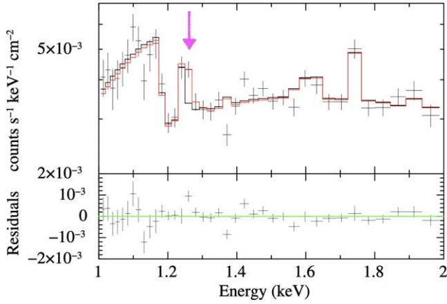
Figure 1. RGS spectrum of GRB 221009A. The data have been normalized by the RGS effective area (set plot area in XSPEC). The absorbed power-law best-fit model is represented with a continuous black line. The best-fit model including the Mg emission line is overplotted in red (to show the minimal change of the continuum). A pink vertical arrow indicates the Mg line energy. Residuals for the power-law model only are shown in the lower panel.
