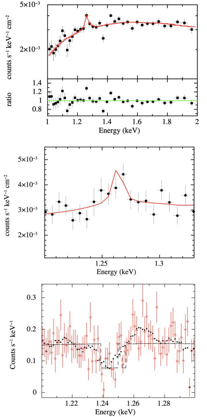
Figure 2. Upper panel: unfolded RGS spectrum of GRB 221009A. The best-fit absorbed power-law best-fit model including the Mg emission line is depicted in red. The ratio plot in the lower panel shows the ratio without the line. Medium panel: zoom of the line energy range with an RGS spectrum rebinned by only a factor of 3 in channels. The best-fit model is in red. Lower panel: original unbinned data (open red points) in the 1.2–1.3 keV together with smoothed (but not binned) data (filled black points) with a Gaussian kernel of 7 eV, equivalent to the RGS FWHM at these energies. The dashed line shows the spectral model with no line. The large dip between 1.24 and 1.25 keV and the small dip just above 1.25 keV are due to the instrument response.
