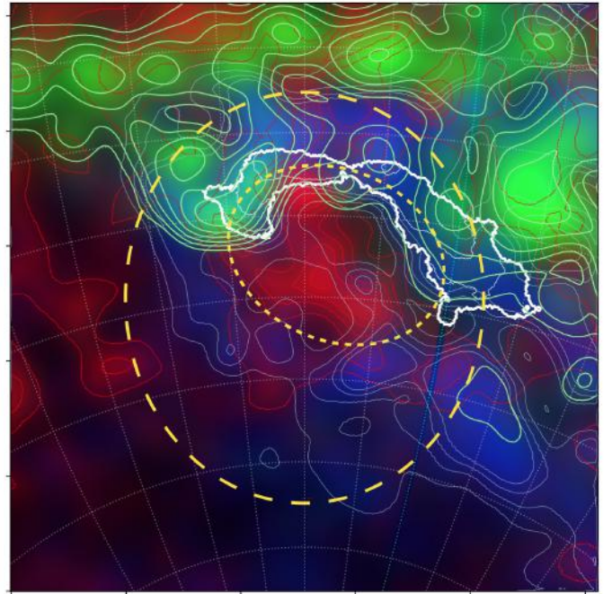
Fig. 5. RGB composite image showing: the 3D dust map integrated between 300 and 500 pc in blue colours and contours as in Fig. 2; the ^{26}\text{Al} emission map from Diehl (2002) in red colours and contours. Red contours are between 2.8 \times 10^{-6} and 2.4 \times 10^{-4} \text{ cm}^{-2} \text{ sr}^{-1} \text{ s}^{-1} in steps of 2.7 \times 10^{-5} \text{ cm}^{-2} \text{ sr}^{-1} \text{ s}^{-1} . The Orion-Taurus ridge is shown with white contours as in Fig. 1; the N_{\text{H}_2} map from Kalberla et al. (2020) is in green colours and contours between 6.3 \times 10^{20} and 10^{22} \text{ cm}^{-2} in \log_{10} -steps of 0.2. The yellow circles are the same as in Fig. 2.
