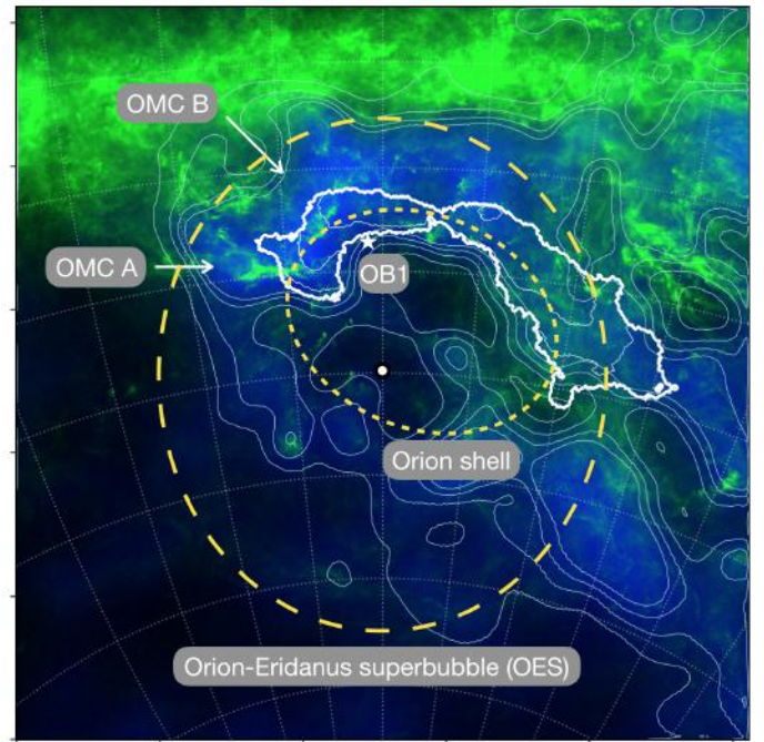
Fig. 2. Stereographic view of the 3D dust map integrated between 300 and 500 pc (in blue) and the total gas column density ( N_H , in green) toward the Orion-Taurus ridge, shown with white contours. Light-blue contours trace the 3D dust map at A_V = 2, 3, 4, 5 \text{ mag} . The N_H map is shown above 10^{21} \text{ cm}^{-2} . The coordinate grid and the white contours are the same as in Fig. 1. The long-dashed yellow line indicates the edge of the OES. The short-dashed-yellow line indicates the edge of the Orion shell reported by Foley et al. (2023). A white circle highlights the center of the OES.
