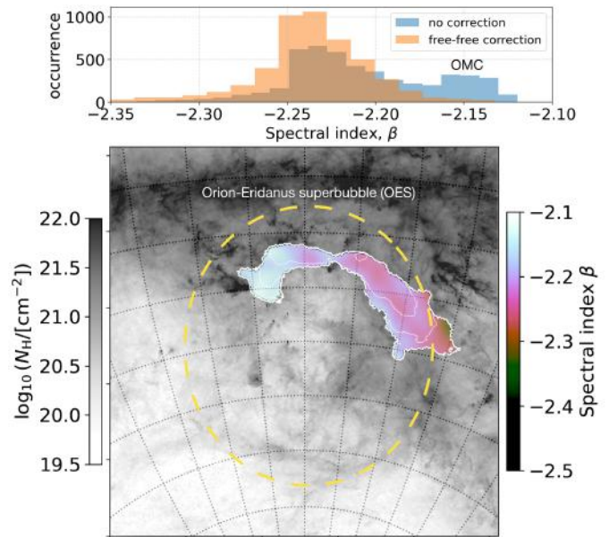
Fig. 4. Synchrotron spectral-index map ( \beta , FWHM \approx 3.5^\circ , colors) of the Orion-Taurus ridge computed using LWA data at 50, 60, 70, 74, and 80 MHz. The \beta map is overlaid on the N_{\text{H}} map from Planck . The inset above shows the histograms of \beta before (blue) and after (orange) free-free absorption correction. The OMC corresponds to the blue peak at \beta = -2.15 .
