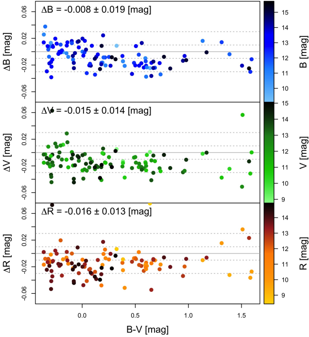
Figure 14. As Figure 13, but comparing with the Johnson-Kron-Cousins magnitudes of the SPSS by Altavilla et al. (2021) . The top panel refers to the B magnitude, the middle one to V, and the bottom one to R, as labelled.
