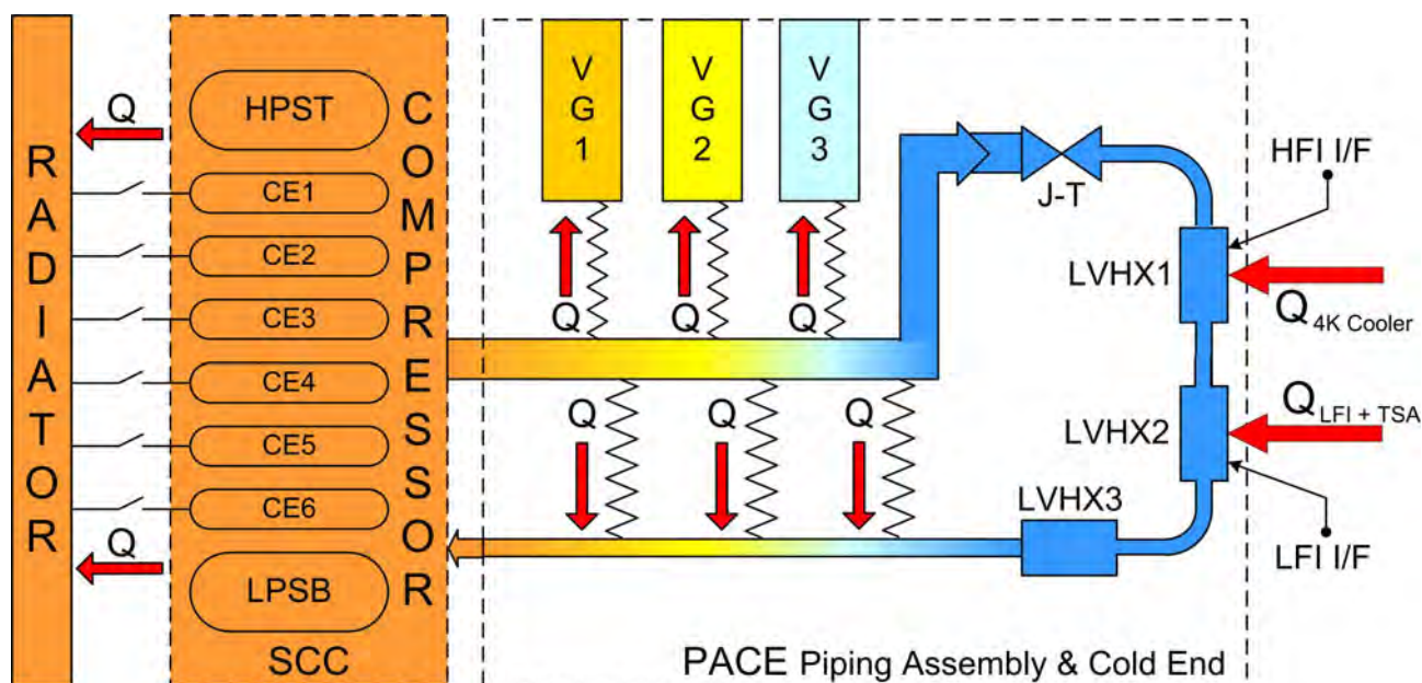
Figure 4-1 TMU thermal configuration
