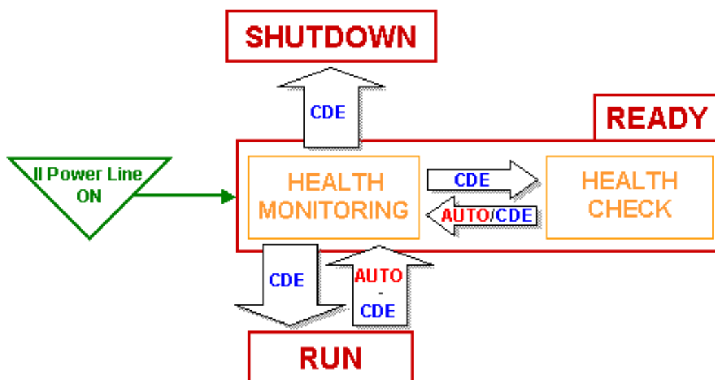
Figure 6-6 READY Mode
