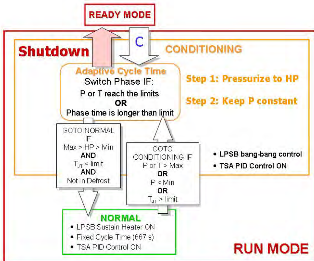
Figure 6-2 RUN Mode Block Diagram
