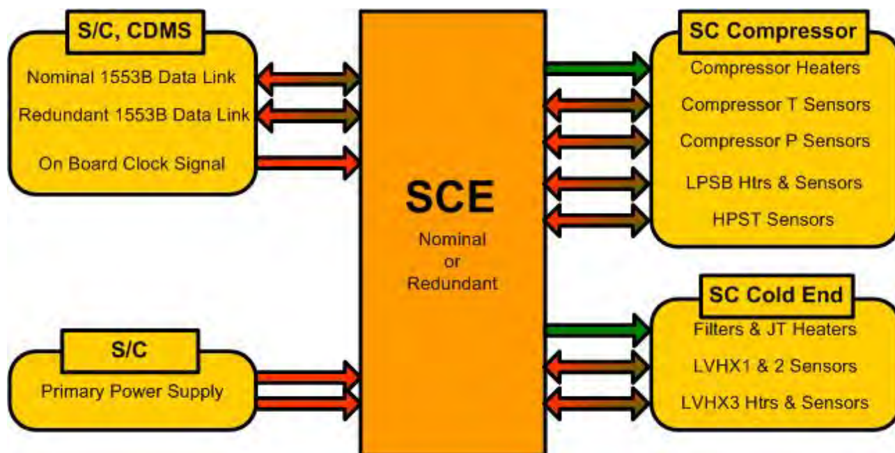
Figure 2-7 SCE electrical interfaces
