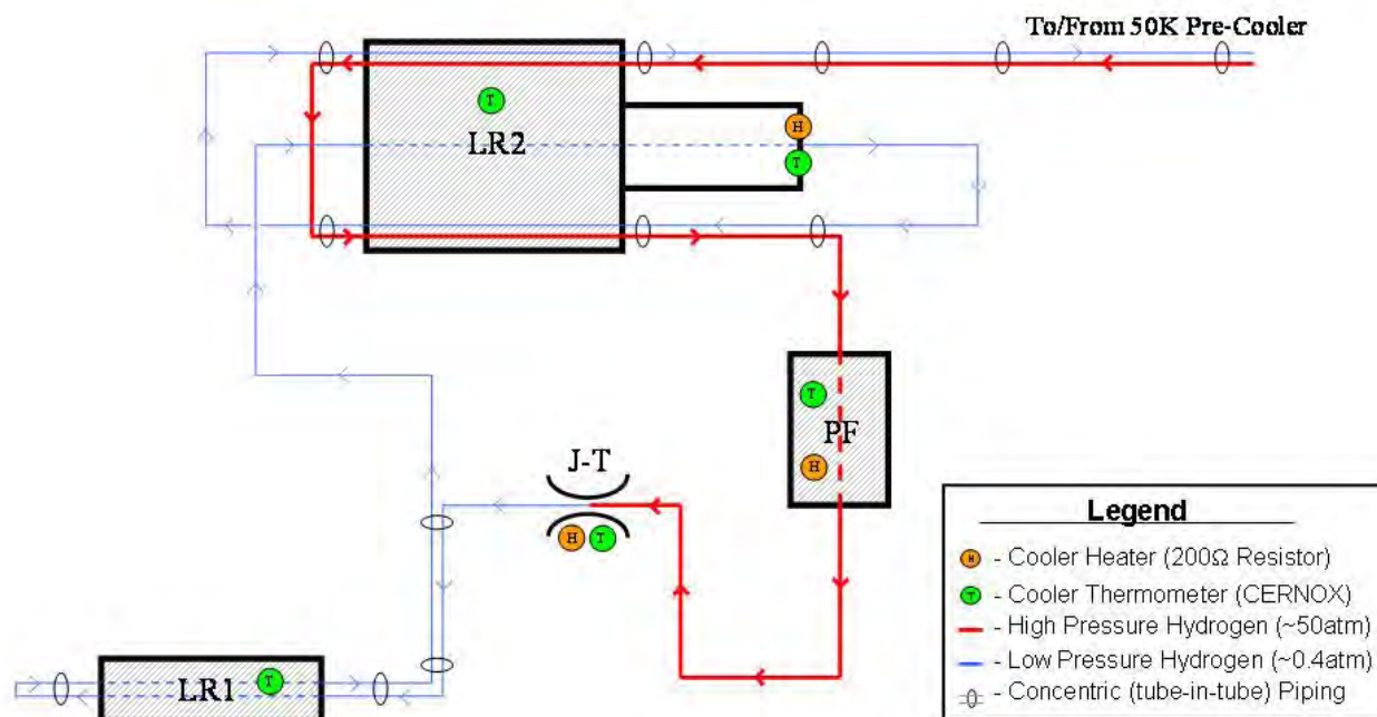
Figure 3-3 SCCE functional description
