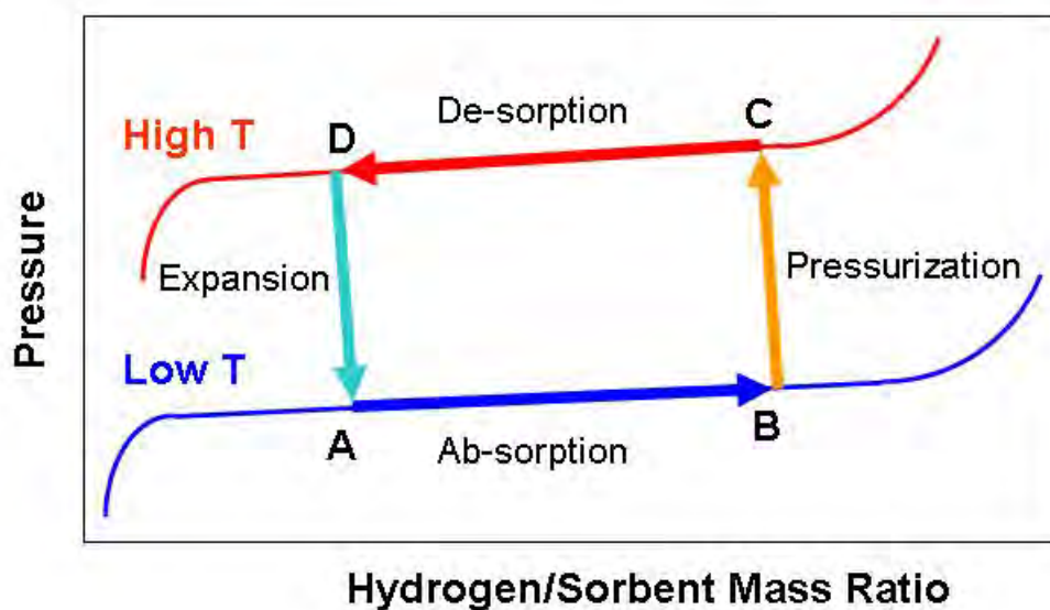
Figure 3-2 Hydride Isotherms
