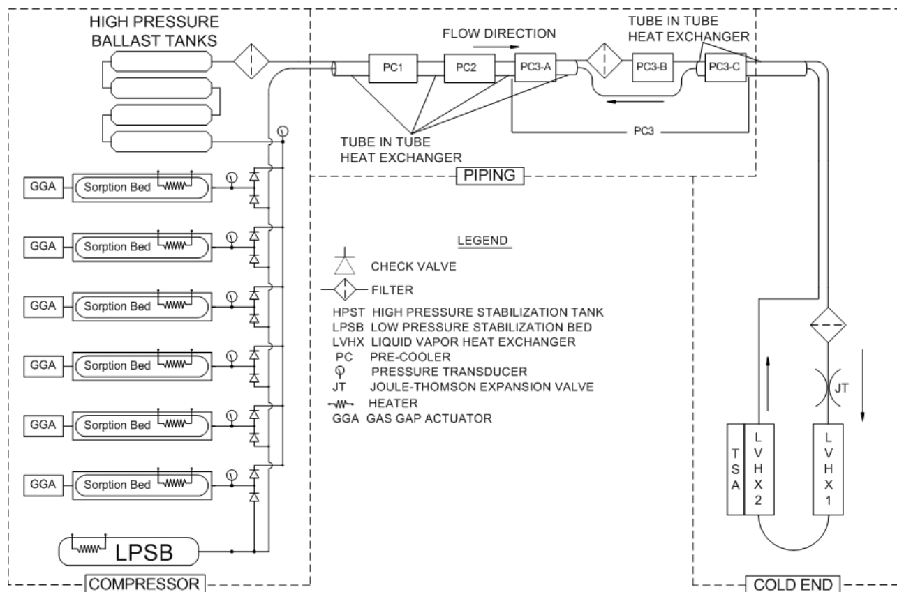
Figure 1-1 TMU schematic
