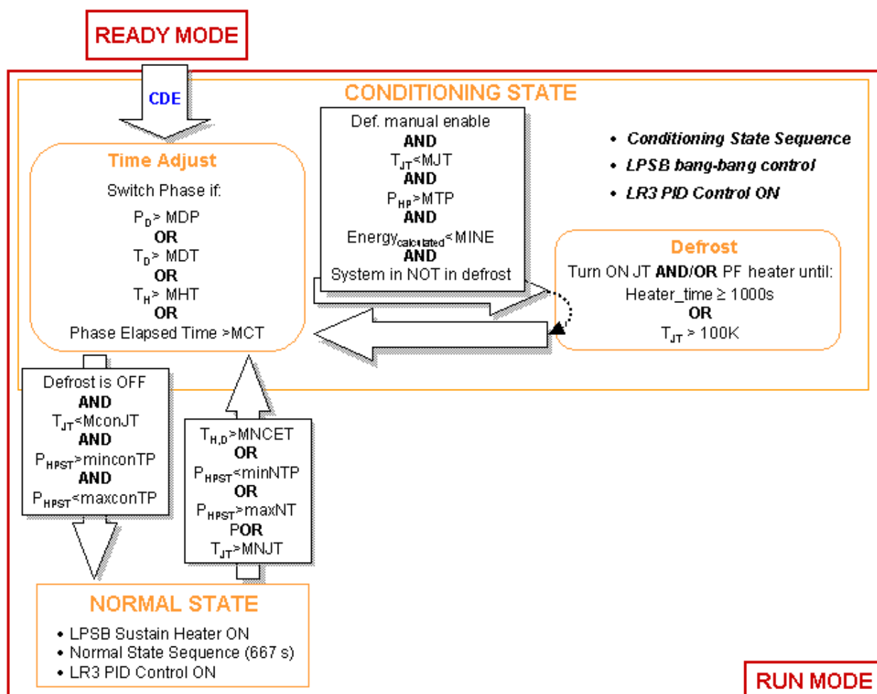
Figure 6-7 RUN Mode
