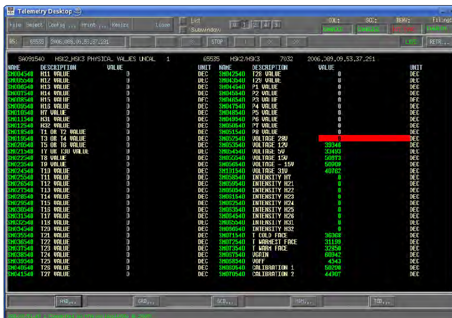
Figure A3-48: The SA091559 AND – Uncalibrated parameters from housekeeping in ASW modes
