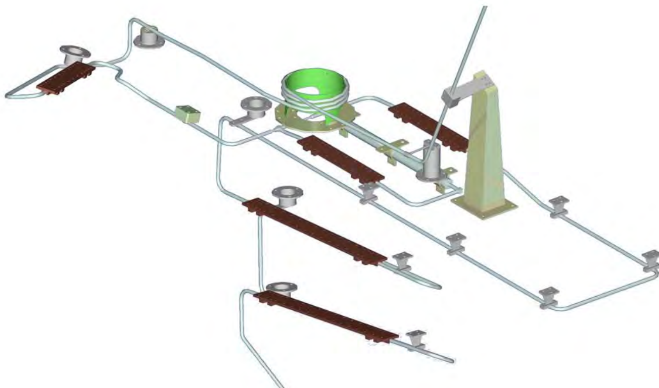
Figure 2-4 Cooler Piping from Compressor to Cold End
