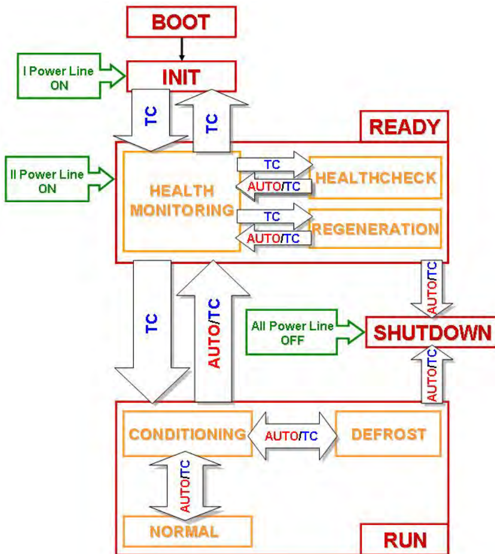
Figure 8-11: Operating Modes
