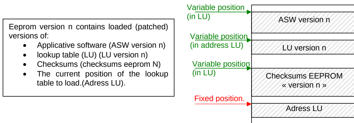
Figure 8-26: Eeprom configuration
