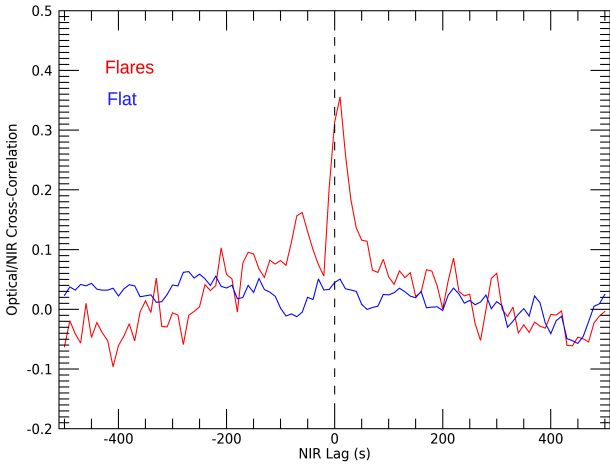
Fig. 6. Optical/NIR CCF computed in two different selected segments of the NIR light curve. A strong peak is present only in the variable part of the light curve. Uncertainties are of the order of 0.05 (68% confidence level).
