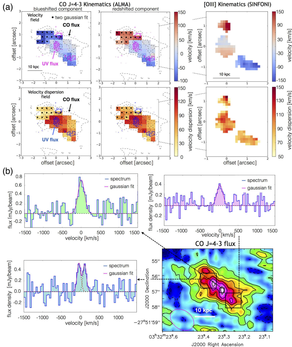
Figure 4. (a) Left-hand panels: CO J=4-3 velocity field and velocity dispersion. Dots indicate regions where a fit with two Gaussian components is required; in these cases the two kinematics components (‘blueshifted’ and ‘redshifted’) are shown separately. The solid contours show the rest-frame UV emission traced by HST . Right-hand panels: velocity field and velocity dispersion of the three galaxies traced by the [O III]5007 Å optical nebular emission line (Maiolino et al. 2008; Troncoso et al. 2014). (b) Bottom right panel: CO J=4-3 surface brightness within the central few tens kpc around Candels-5001 (same levels as Fig. 3a). Top/bottom left panels: spectra extracted from the central region and from two outer regions, one of the latter showing indication of a double-peaked profile.
