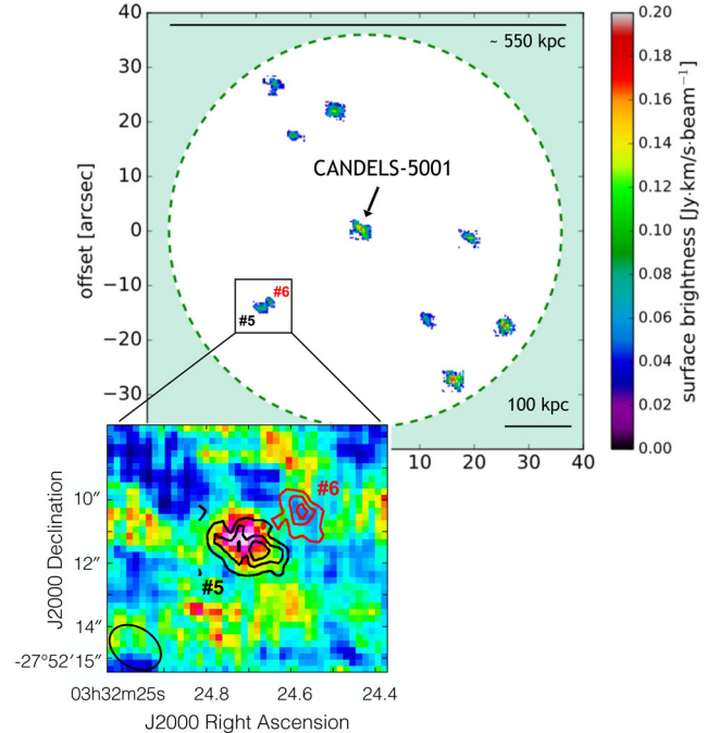
Figure 8. Distribution of CO-emitting systems detected on the 550 kpc scale around Candels-5001. The dashed circle encloses the region where the primary beam response function is above 30 per cent. The image of each object is shown down to the 1\sigma level of the CO surface brightness. The inset shows (in colour) the ALMA continuum emission map for the galaxy (in addition to Candels-5001 and its surrounding 40 kpc) clearly detected in continuum. Black and red contours show CO emission systems no. 5 and no. 6 (see Appendix D), respectively, at levels of 2\sigma , 3.5\sigma and 5\sigma .
