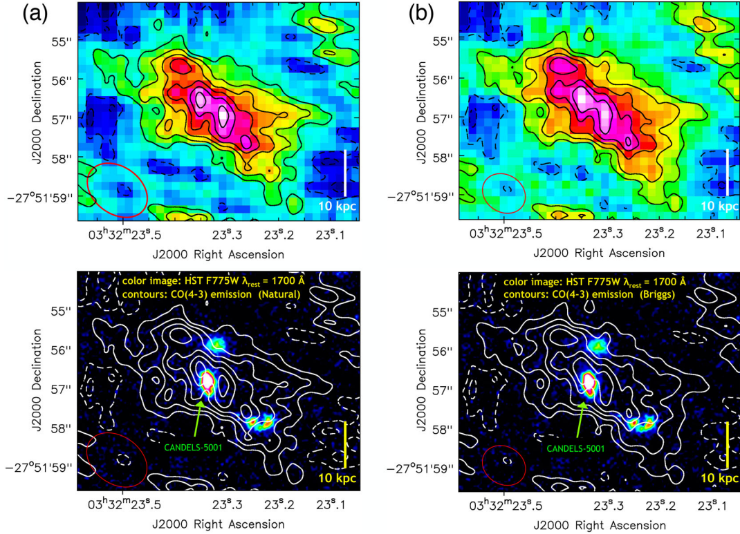
Figure 3. (a) Upper panel: CO J=4-3 map of the region around Candels-5001 obtained through natural weighting of the visibilities. The CO surface brightness contours range from 1\sigma to 6\sigma , where \sigma = 22 \text{ mJy km s}^{-1} \text{ beam}^{-1} is the CO map rms. Dashed contours indicate negative fluxes. Lower panel: the same CO contours are shown overlaid on to the F775W HST image (colour). (b) Upper panel: CO J=4-3 map obtained through the Briggs weighting (robustness parameter: +2). Contours range from 1\sigma to 5\sigma , where \sigma = 24.5 \text{ mJy km s}^{-1} \text{ beam}^{-1} . In this image, the extended emission is even more clearly resolved, over more than 10 independent beams, although the sensitivity is somewhat lower. Lower panel: same background colour image of (a), with surface brightness contours of CO J=4-3 Briggs weighted map overlaid. The beam sizes of the ALMA maps are given in the bottom-left corners.
