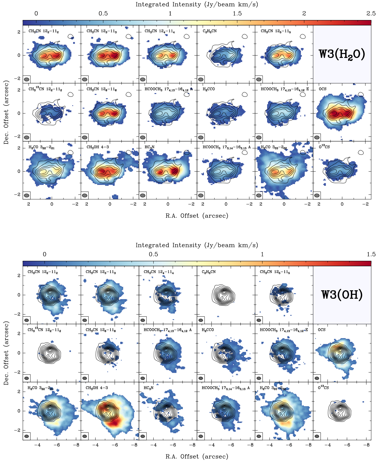
Fig. A.1. Integrated intensity (zeroth moment) maps of most important lines covered in the narrow-band receiver for the observations in the ABD configuration for W3(H 2 O) ( top panel ) and W3(OH) ( bottom panel ). The solid contours correspond to the dust continuum and start at and increase by 6\sigma ( 1\sigma = 3.2 \text{ mJy beam}^{-1} ). The size of the synthesised beam is shown in the bottom left of each panel. The map of CH 3 CN ( 12_5-11_5 ) may not be accurate because it is blended with other lines.
