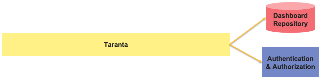
Figure 3. Taranta Services
