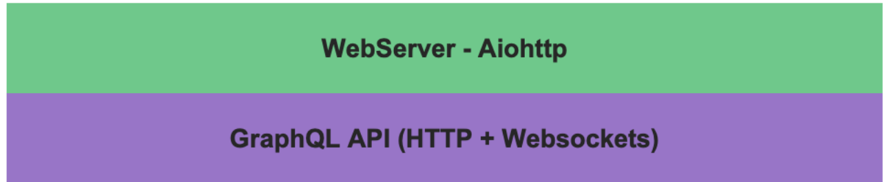
Figure 4. Taranta Backend
