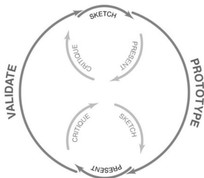
Figure 6. LeanUX Process
