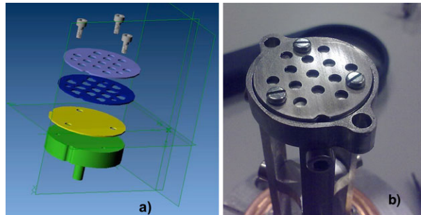
Fig. 3 (a) Collector exploded view. The three parts are linked together by 3 screws, once fixed with the base the holes of the first disk constitute the hollow where the TEM GRIDS will be housed, the holes of the second disk are concentric with the holes of the first but with a diameter smaller than the diameter of the TEM grids to lock them inside the sample holder. (b) DUSTER collector in final configuration
