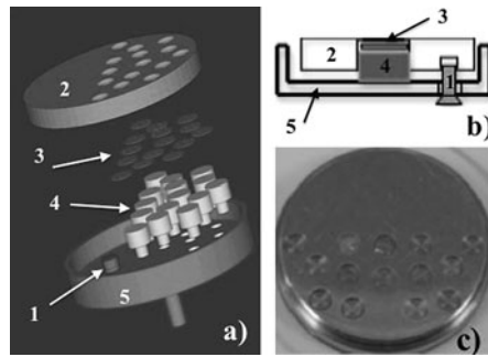
Fig. 2 Duster 2008 collector: (a) 3D exploded view; (b) scheme and (c) image of the assembled view. In panel (a) and (b): (1) screw fixing the gold plated holed mask to the external stainless steel frame; (2) gold plated holed mask; (3) Transmission Electron Microscope grids; (4) stainless steel pins; (5) external stainless steel frame of the assembly. The collector dimensions are: diameter of the gold holed mask = 23 mm, total diameter of the collector = 24.5 mm, total height of the sample holder = 16 mm, diameter of the holes in the gold mask = 2.46 mm, diameter of the TEM grids = 3.05 mm
