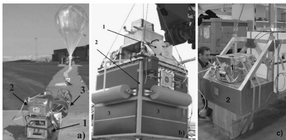
Fig. 10 (a) DUSTER 2008 in the stand-alone flight configuration: (1) DUSTER; (2) ASI Telemetry System; (3) Solar panels fixed along the chain. (b) DUSTER 2009 in the piggy-back flight configuration on the SORA main payload, pending from the crane: (1) DUSTER; (2) SORA gondola; (3) DUSTER Solar panels. (c) DUSTER 2011 in a shared gondola flight configuration: (1) DUSTER; (2) CNES multi-instrument host gondola
