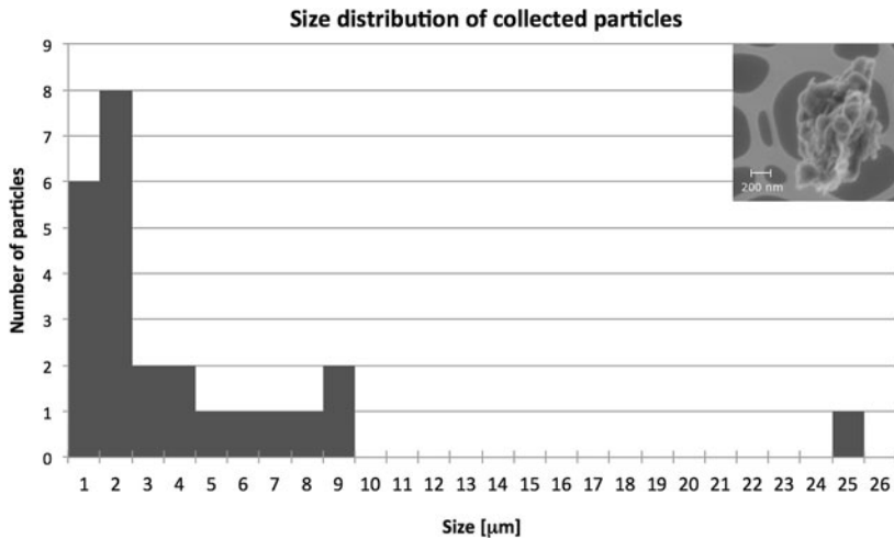
Fig. 15 Size distribution of the 25 identified particles from the Duster 2008 collection. In the insert is shown as an example a SEM image of one of the 25 particles collected in the flight
