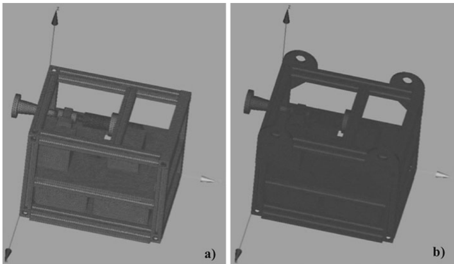
Fig. 7 (a) DUSTER Finite Element Analyses model in piggyback configuration and (b) DUSTER Finite Element Analyses model in the stand-alone configuration with the reference frame
