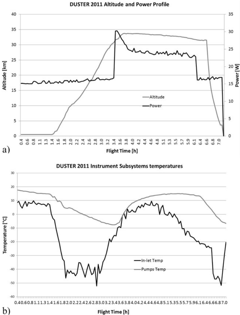
Fig. 14 (a) Altitude and power (sampling) profile for DUSTER 2011 flight. (b) DUSTER temperature profile measured at the in-let and at the pumping system during 2011 flight
