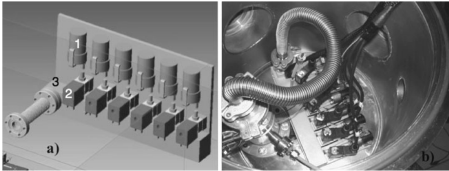
Fig. 4 (a) Pumping system mechanical configuration: (1) pump, (2) micro electro-valve, (3) connecting pipe; (b) The pumping system in the climatic chamber simulating stratospheric conditions of pressure and temperature to measure the flow rate
