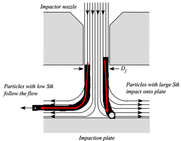
Fig. 1 A schematic view showing the interaction between air flow and mechanical elements which allows the aerodynamic separation and collection of solid phase dispersed in the gas
