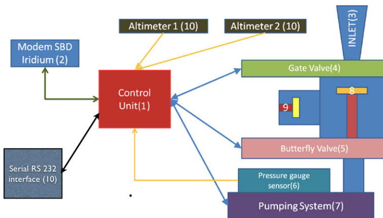
Fig. 8 DUSTER block diagram: (1) Control Unit; (2) IRIDIUM Transceiver; (3) INLET pipe exposed to atmosphere; (4) Gate valve connecting INLET to collecting chamber; (5) Butterfly valve between collecting chamber and pumping system; (6) Pressure gauge monitoring flow through the instrument; (7) Pumping System with 6 micro-pump carbon vane; (8) Collecting substrate; (9) Contamination control substrate; (10) Serial RS 232 interface; (11) GPS antenna
