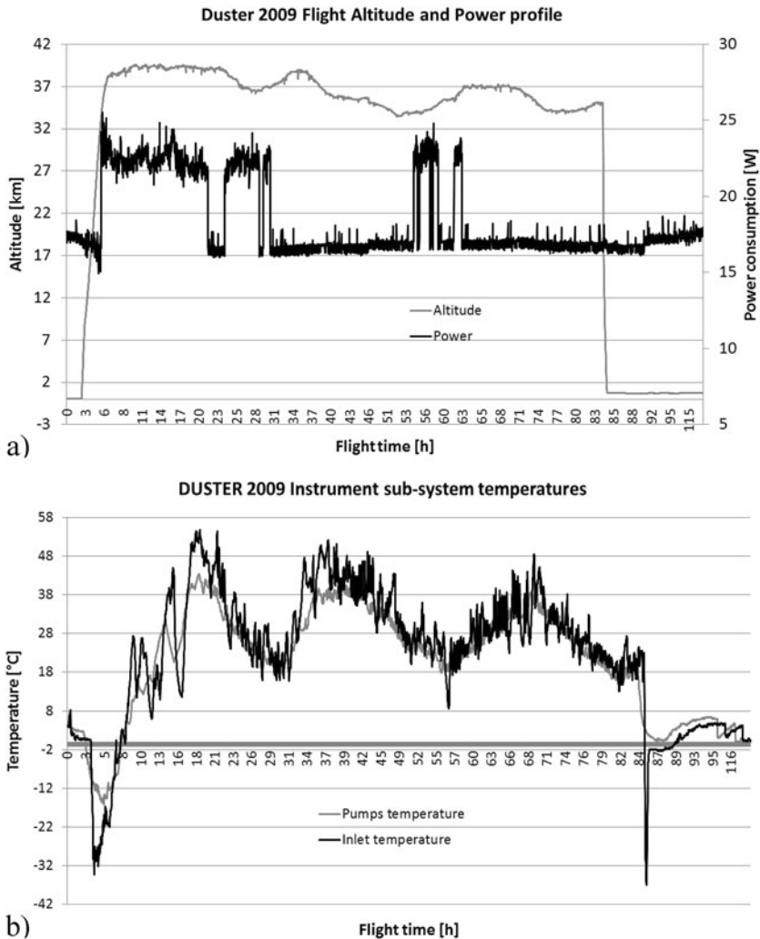
Fig. 13 (a) Altitude and power (sampling) profile for 2009 flight. (b) DUSTER temperature profile measured at the in-let and at the pumping system during 2009 flight
