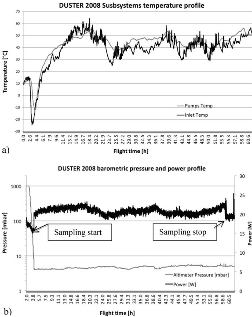
Fig. 12 (a) DUSTER temperature measured at the in-let and at the pumping system during the 2008 flight; (b) Altimeter readings and power consumption profile for the 2008 DUSTER flight
