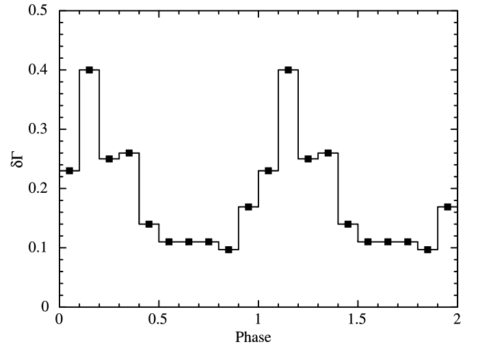
Fig. 12. LS 5039: one sigma uncertainty on the spectral index obtained for 10 h observations per orbital bin.
