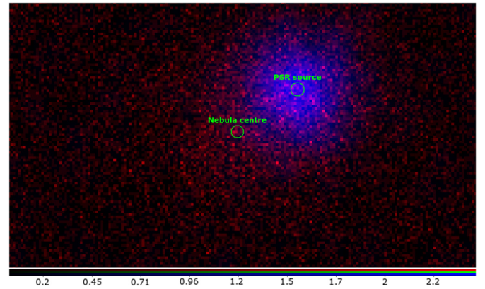
Fig. 20. Colour map for the energy-dependent (red and blue, respectively) are over-imposed. Circles around the position of the PSR source and for the extended Nebula show the positional uncertainties as derived from a maximum likelihood fit. Colour map units are counts/pixel.
