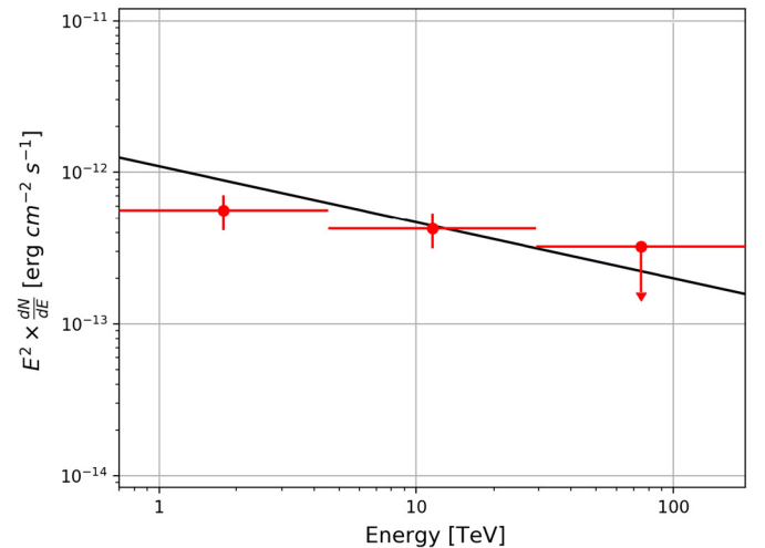
Fig. 10. Examples of simulated spectra of the East e1 hot-spot of SS433 (100 hr). Data points are at a 3\sigma threshold. Left: spectrum assuming source morphology as point-like. Right: assuming extended source morphology ( 0.25^\circ size). Best-fit power-law models shown as thick black lines.
