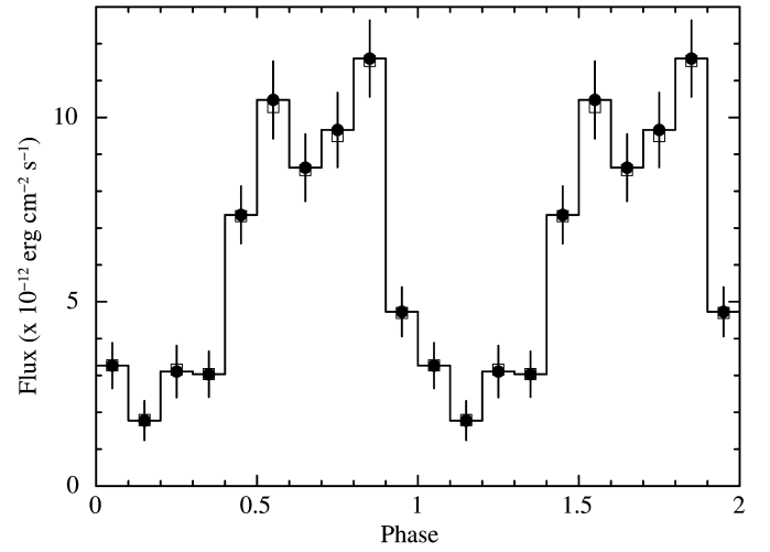
Fig. 11. LS 5039: orbital modulation obtained with 10 h observation per bin. The open squares are the expected fluxes from the simulated models while the filled circles are the obtained flux in 0.8–200 TeV with error bars at one sigma.
