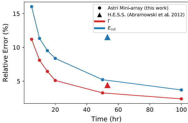
Fig. 17. Relative error of the photon index \Gamma (in red) and cut-off energy E_{\text{cut}} (in blue) as a function of the total observation time for the ASTRI Mini-Array simulations (dots). H.E.S.S. constraints are shown here for comparison as triangles.
