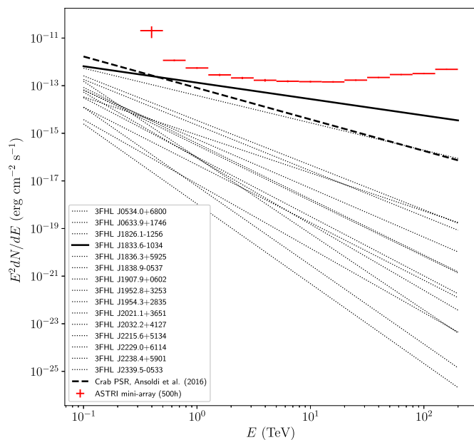
Fig. 7. Spectral energy distribution of pulsars observable from the northern hemisphere over-imposed to the ASTRI Mini-Array 500 h sensitivity curve. Pulsar spectra are taken from the Third Catalogue of Hard Fermi -LAT Sources (3FHL) and extrapolated up to 200 TeV.
