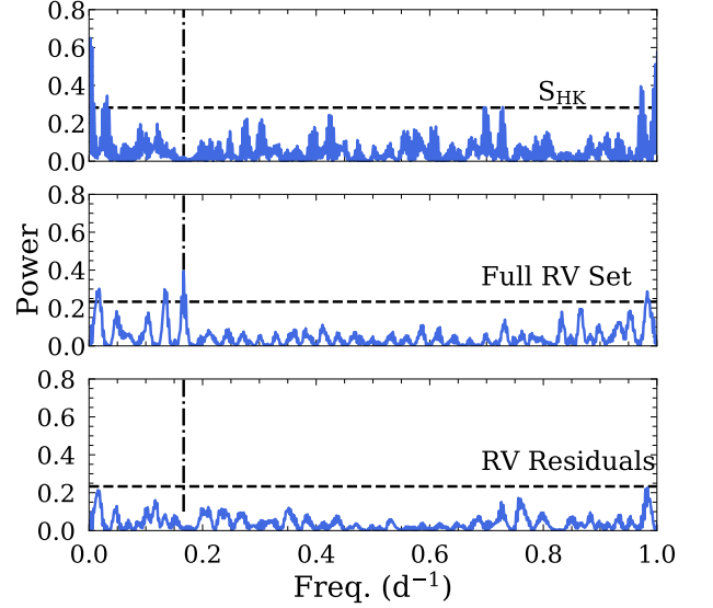
Figure 5. Generalized Lomb-Scargle periodograms of all S_{HK} measurements (top), the full radial velocity data set (middle) and the RV residuals after the subtraction of a 1-planet fit (bottom). The dashed horizontal lines represent the power needed to attain a false alarm probability of 0.1% while the vertical dashed-dotted line marks the period of the planet. Although there are prominent peaks seen in the S_{HK} periodogram these peaks are not seen in the full data set.
