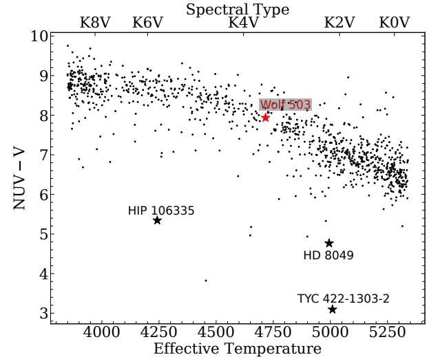
Figure 6. NUV-V colors and effective temperatures for nearby (within 50pc) K-dwarfs from the TESS Input Catalog. Most stars are in a quiescent group signifying low NUV emission while some stars are outliers. A number of these outliers (e.g HIP 106335, HD 8049) are known to have higher stellar activity. Wolf 503 (red star) is a member of the quiescent group which agrees with measurements of stellar activity such as S_{HK} .
