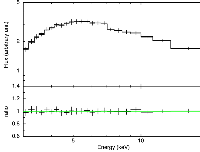
Figure A2. Median rest-frame spectrum from the simulated Chandra and NuSTAR spectra with \Gamma = 1.8 and N_H = 10^{23} \text{ cm}^{-2} . To test the reliability of our averaging method and constrain the underlying continuum, the median spectrum was fitted with an absorbed power-law model between 3 and 30 keV: we recovered the input photon index \Gamma = 1.8 and N_H = 10^{23} \text{ cm}^{-2} with a scatter of \sim 1\% and \sim 2\% respectively. The bottom panel shows the ratio between the simulated data and the model.
