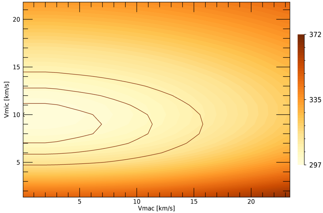
Supplementary Figure 6. \chi^2 minimization map of the LTE synthetic spectrum with contour lines of 1 \sigma , 2 \sigma and 3 \sigma confidence intervals for the values of the microturbulence ( v_{\text{mic}} ) and macroturbulence ( v_{\text{mac}} ) velocities.
