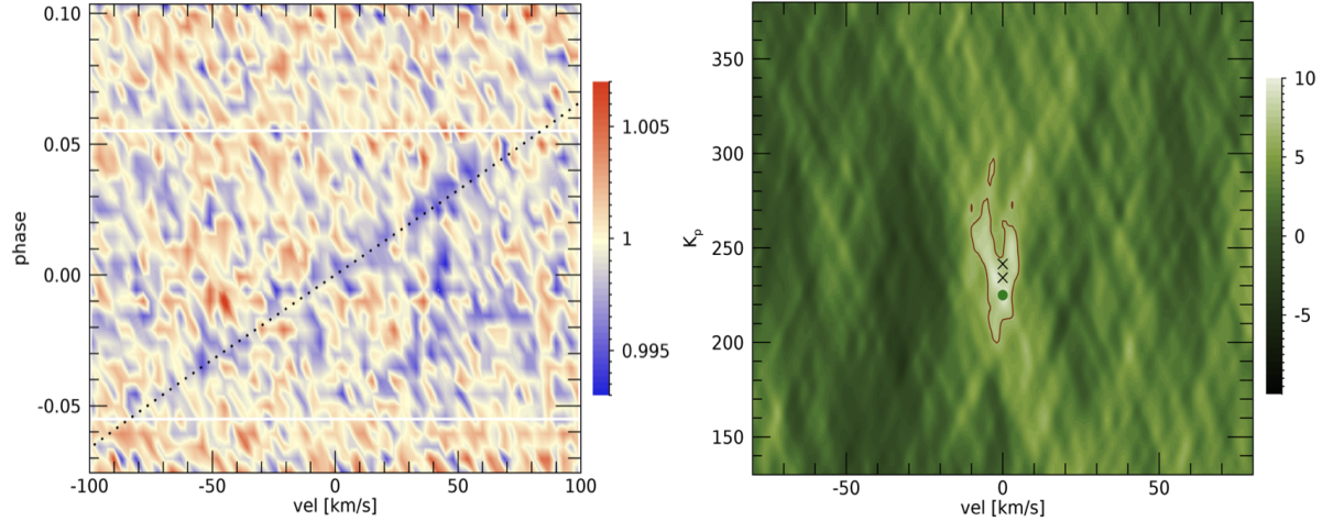
Figure 2. a , 2D contour map of the oxygen triplet averaged in velocity space, in the stellar rest frame. The black dotted line shows the expected motion of the planetary signal. The white horizontal lines mark the beginning and end of the transit. The colour scale shows the relative flux variation. b , K_p - V_{\text{sys}} map for the OI triplet. Crosses mark the position of the K_p (the RV semi-amplitude of the planetary Keplerian motion) determined by Refs. 14,15 . The green dot marks the best K_p position in the map. The solid line shows the 3\sigma confidence interval. The colour scale shows the signal-to-noise ratio of the detection.
