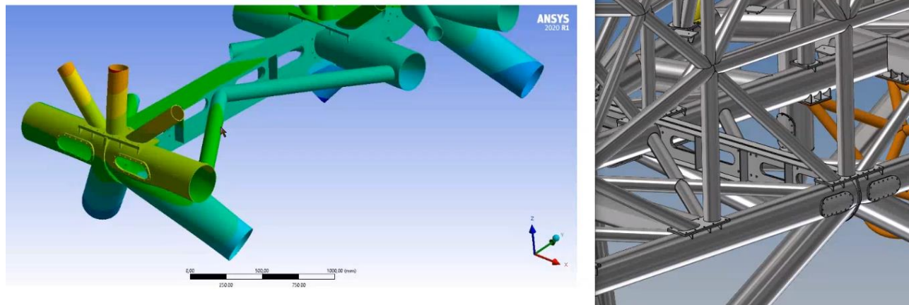
Figure 12. MAORY MSS Results - Local stress analyses.
