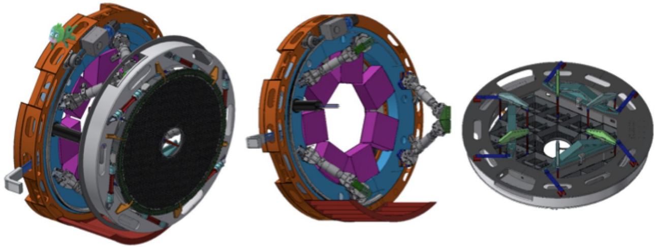
Figure 2. A figure of M4 unit (left) and its two main parts hexapod platform (center) and reference and optical surface (right). The CalUnit hardware can be located in between (a) and (b).
