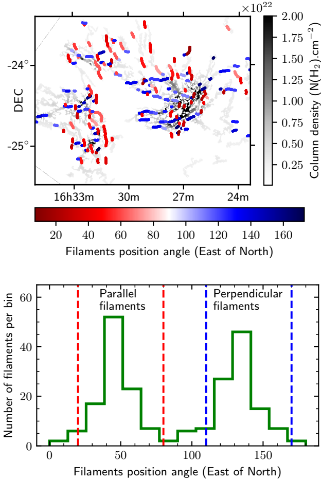
Fig. 10. Top: skeleton map of filament orientations (colorscale) overlaid on a filtered version of the Herschel column density map of the Ophiuchus cloud (grayscale) obtained with the getfilaments algorithm (see Fig. 7). The filamentary structures identified with getfilaments are displayed in red or blue depending on their position angles measured east of north (see colorscale). Bottom: distribution of median position angles (PA) for the sample of filaments identified with getfilaments (cf. Sect. 4.3). Two modes of filament orientations are clearly visible. The “parallel” filaments (with PA from 20 to 80 degrees east of north) are following the general direction of the large-scale streamers (cf. Fig. 1) and may be associated with material swept-up by the winds of the Sco OB2 association (whose general direction is about 45 degrees east of north), while the “perpendicular” filaments (with PA from 100 to 160 degrees) may have formed as a result of large-scale compression from the Sco OB2 winds.
