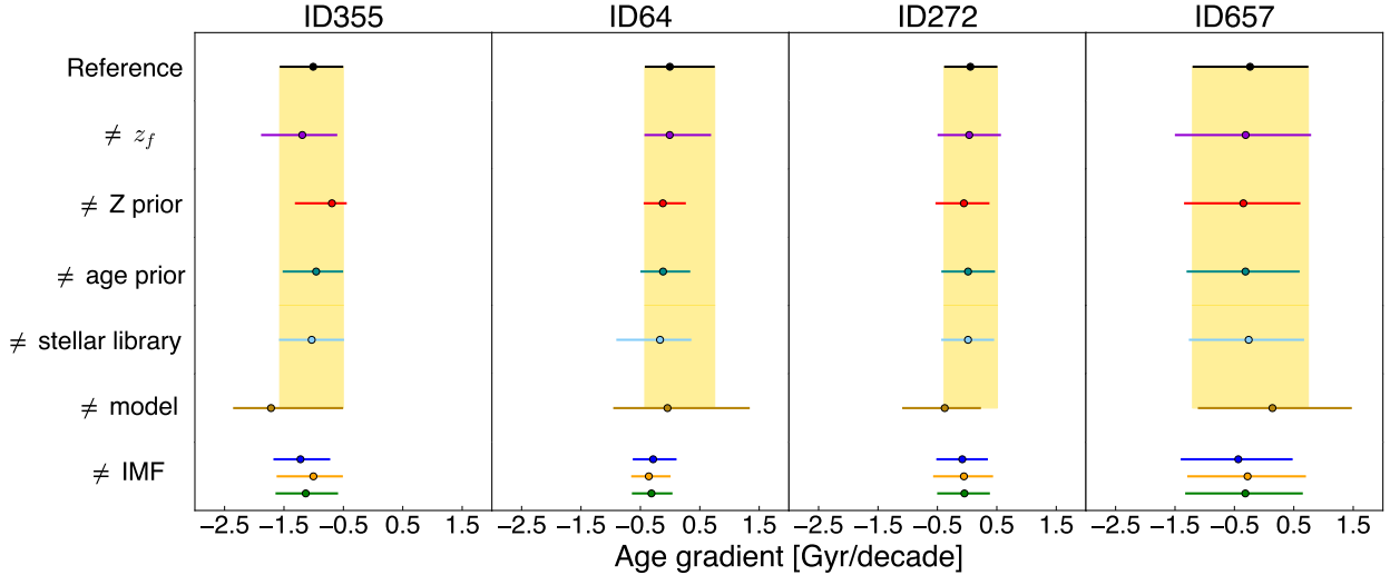
Fig. 11: Sensitivity analysis for the age gradients, colour-coded as in Fig.10.
