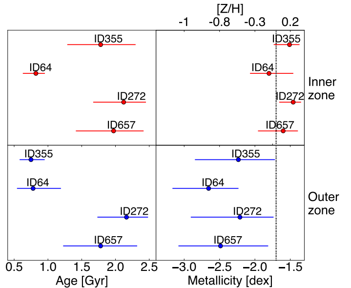
Fig. 8: Age (left panel) and metallicity (right panel) median values in the inner and outer zones of the sample. Solid lines show the 1\sigma errors. The vertical dashed line indicates solar metallicity.
