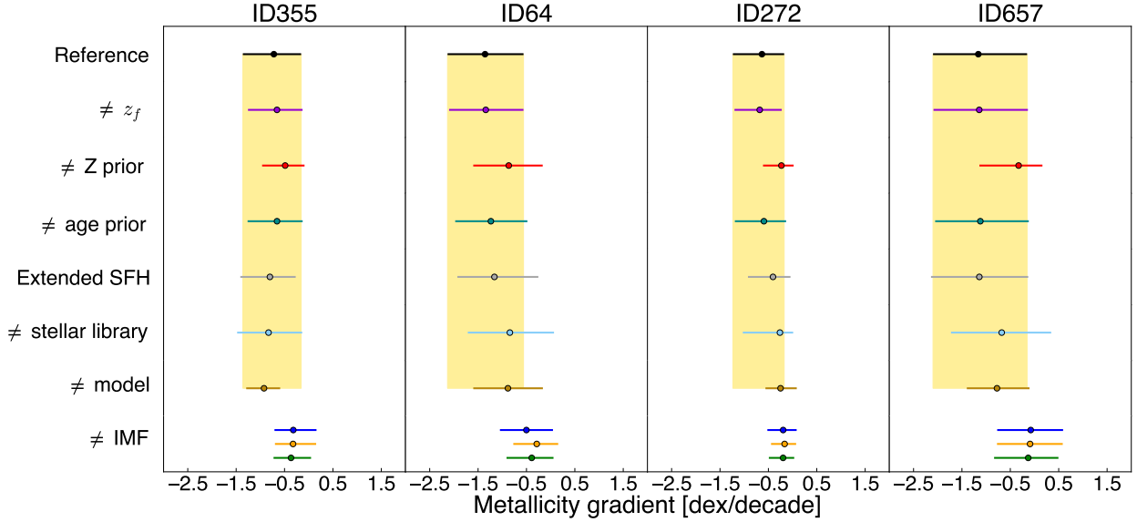
Fig. 10: Sensitivity analysis for the metallicity gradients. The reference analysis (black) adopts BC03 models, the MILES stellar library, a Chabrier IMF, and z_f = 6 . The result we obtained when we adopted a different z_f = 11 is reported in violet, a different metallicity prior (uniform) in red, a different age prior (logarithmically uniform) in cyan, an extended star formation timescale (0.5 Gyr) in grey, a different stellar library (STELIB) in light blue, and a different model (Maraston) in brown. The blue, yellow, and green symbols are gradients derived by adopting a different IMF (−1.5 slope, Salpeter, and −3.5 slope, respectively). These slopes are systematically flatter because the range of metallicities considered in this comparison is smaller.
