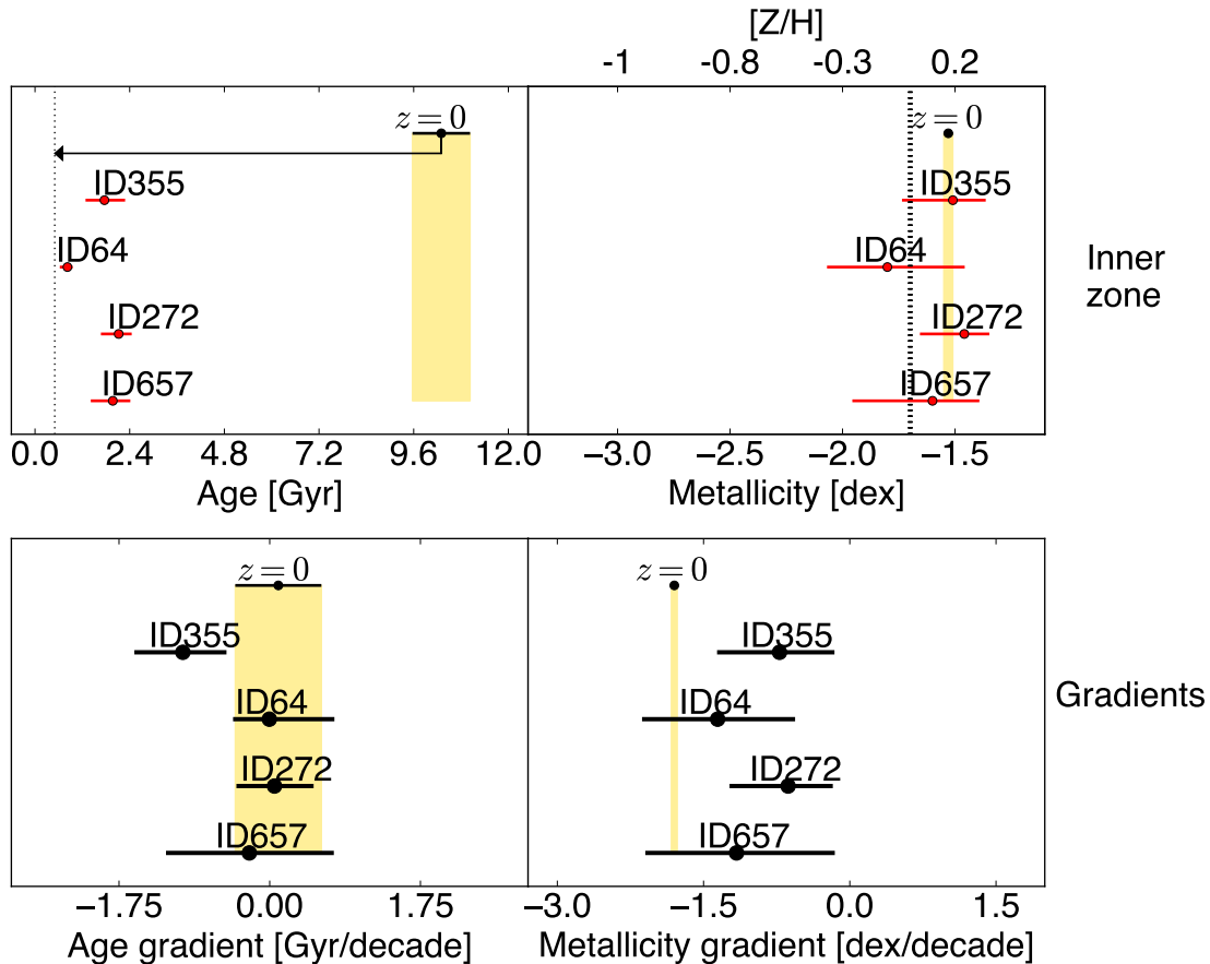
Fig. 12: Comparison between results for the local Universe (Mehlert et al. 2003) and our stellar age and metallicity parameters in the inner zone and their gradients. The arrow in the upper left panel indicates the lookback time between z = 0 and z = 1.8 . The vertical dashed line indicates solar metallicity.
