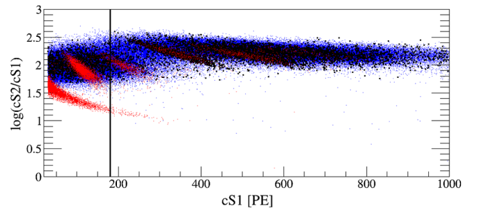
FIG. 9. The full XENON100 dark matter science run data up to 1000 PE in cS1 (shown in black). In blue, we show data from ER calibration ( ^{60}\text{Co} and ^{232}\text{Th} ), and in red, we show data from NR calibration ( ^{241}\text{AmBe} ). See the text for details on these populations. While the black vertical line represents the highest energy considered for quantitative interpretation in this analysis, there is no indication of elastic NRs even above that energy.
