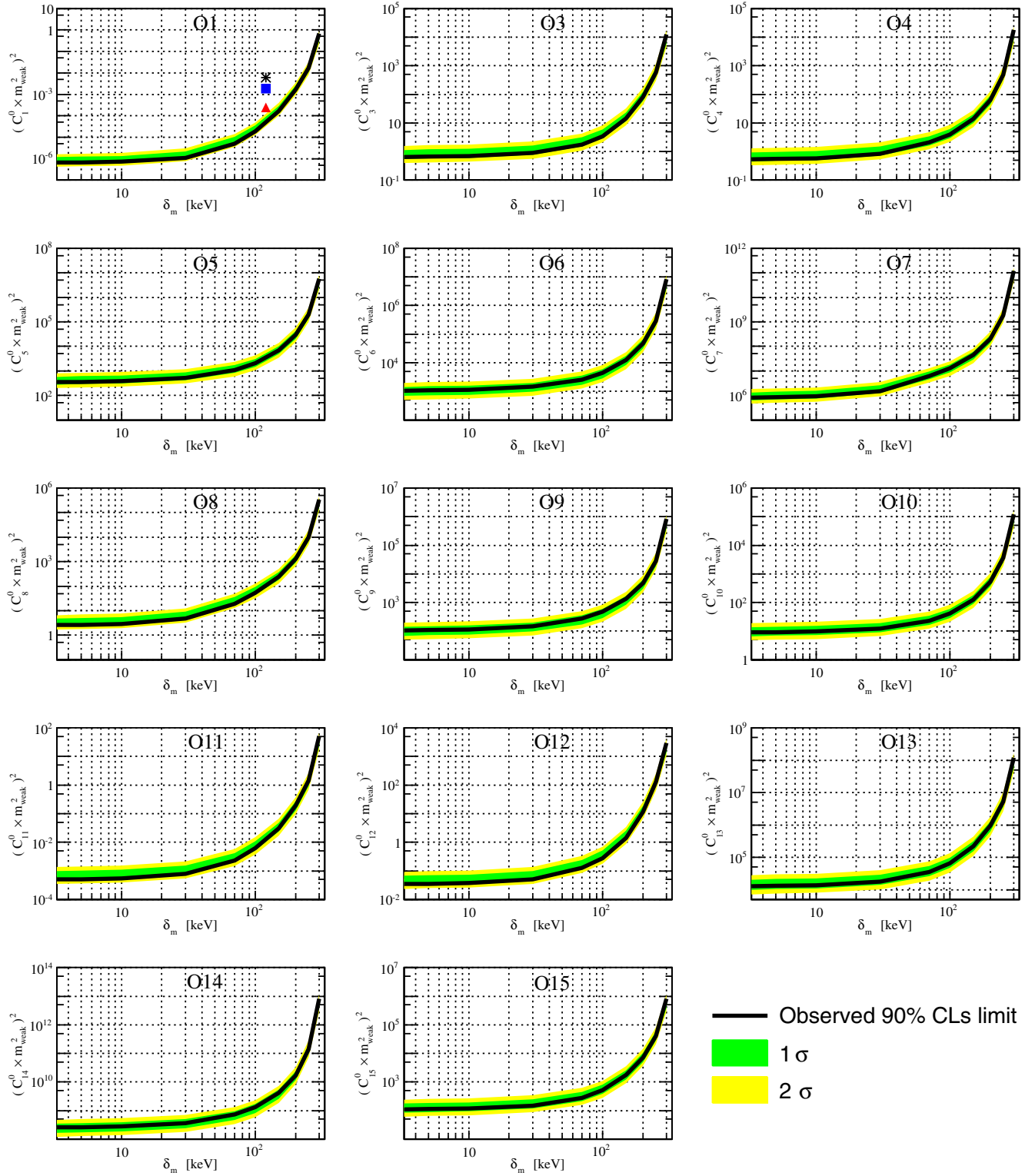
FIG. 8. The XENON100 90% C.L.s limits on a 1 TeV/ c^2 WIMP isoscalar dimensionless coupling constant as a function of the WIMP mass splitting \delta_m for all inelastic scattering EFT operators. Limits are indicated in solid black. The expected sensitivity is shown in green and yellow ( 1\sigma and 2\sigma , respectively). For \mathcal{O}_1 , (SI) results from XENON100 (red triangle), CDMS-II (blue rectangle), and ZEPLIN-III (black star) are overlaid.
