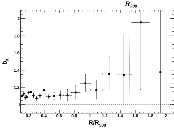
Figure 7. Average emissivity bias b_X (left, see Eq. 1) and clumping factor \sqrt{C} (right, see Eq. 2) as a function of distance from the cluster center for our sample of 31 clusters.
