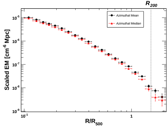
Figure 6. Median self-similar scaled emission-measure profiles obtained using the standard way (black circles) and by applying the azimuthal median technique presented here (red triangles).
