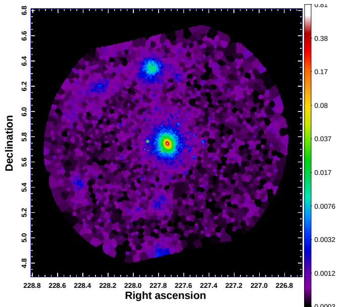
Figure 4. ROSAT /PSPC surface-brightness image of A2029 obtained using Voronoi tessellation (Cappellari & Copin 2003), in units of \text{cts s}^{-1} \text{arcmin}^{-2} . Each Voronoi bin includes an average of 20 counts.
