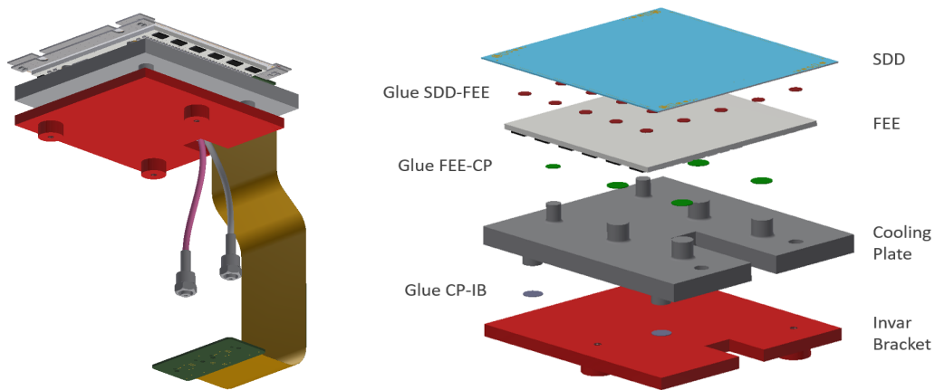
Figure 10. WFM detector assembly (DA). Left panel: layout of the detector assembly, with, from top to bottom, the FEE PCB (Printed Circuit board) including the ASICs and all the FEE components), the cooling plate (gray) and the Invar Bracket (red). The HV (high voltage) and MV (medium voltage) cables are also shown, as well as the flex-print to the BEE. Right panel: scheme of the four layers of the DA, with indication of the glue spots to assembly the corresponding layers one with each other.
