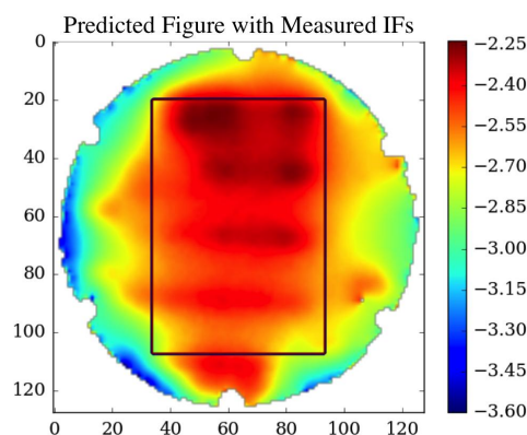
Figure 11. The residuals predicted by the correction algorithm for a 0.1\text{ }\mu\text{m} , 0.06\text{ mm}^{-1} sinusoid input figure using measured influence functions. The color scale is in \mu\text{m} .
