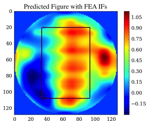
Figure 10. The residuals predicted by the correction algorithm for a 0.1\text{ }\mu\text{m} , 0.06\text{ mm}^{-1} sinusoid input figure using FEA modeled influence functions. The color scale is in \mu\text{m} .
