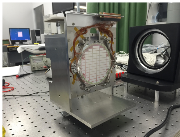
Figure 5. The DFC sample bonded into a six point flexure mount.
