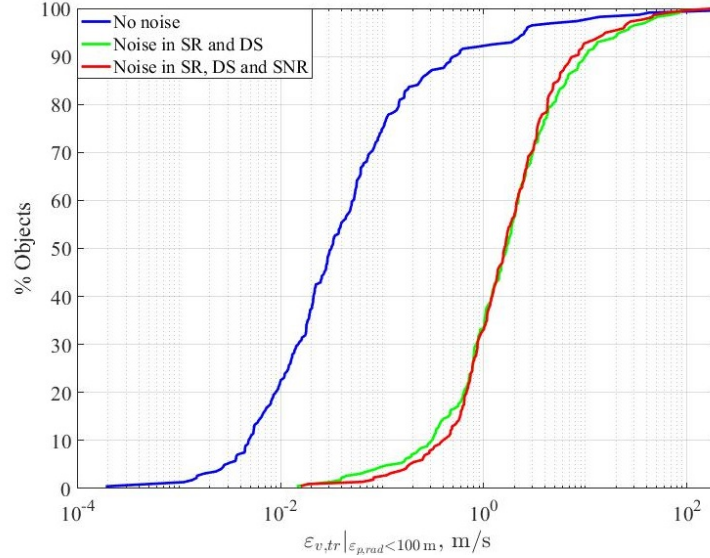
Fig. 12 Cumulative error in transversal velocity for all objects with \varepsilon_{p,rad} lower than 100 m (unknown object, standard configuration).
