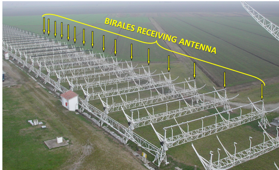
Fig. 3 BIRALES receiving antenna
