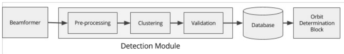
Fig. 6 The main stages of the BIRALES Data Detection Module
