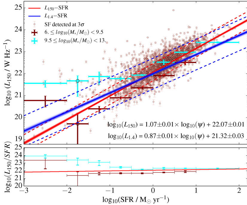
Figure 4. Top: The distribution of LOFAR 150-MHz luminosities of SFGs detected at 150 MHz as a function of their SFRs. The best fit obtained using all SFGs and LOFAR 150-MHz luminosities and errors on the best fit are shown as red shaded region and the blue shaded region shows the best fit to all data points of SFG obtained using L_{1.4} and scaled to 150 MHz assuming \alpha = 0.8 . The dashed lines around the best fits show the dispersion around the best-fitting line implied by the best-fitting dispersion parameter \sigma . The results of the stacking analysis for two stellar mass bins are also shown for L_{150} as large cyan and maroon crosses. Open circles indicate the bins in which sources were not detected significantly. Bottom: The L_{150} -SFR ratios for two stellar mass bins are shown as cyan and maroon crosses, and the best fit divided by the SFR (red line) are shown.
