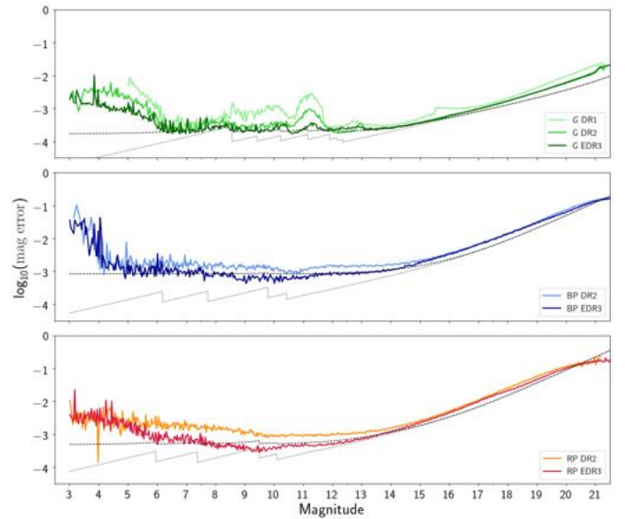
Fig. 14. Distribution of the uncertainty on the weighted mean G (top panel), G_{BP} (central panel), and G_{RP} (bottom panel) as a function of the G , G_{BP} , and G_{RP} magnitude, respectively. Only sources with \approx 20 transits (corresponding to \approx 200 CCD observations in G ) have been included in this analysis. The black dotted line shows the expected uncertainties for sources with 200 G -band (20 G_{BP} , G_{RP} ) contributions for a nominal mission with no calibration error. The dashed dark line shows the same expected uncertainties with an additional calibration error on the single measurement of 2.0 mmag for G -band, 3.1 mmag for G_{BP} and 1.8 mmag for G_{RP} added in quadrature. The Gaia DR1 and DR2 uncertainties are shown for comparison.
