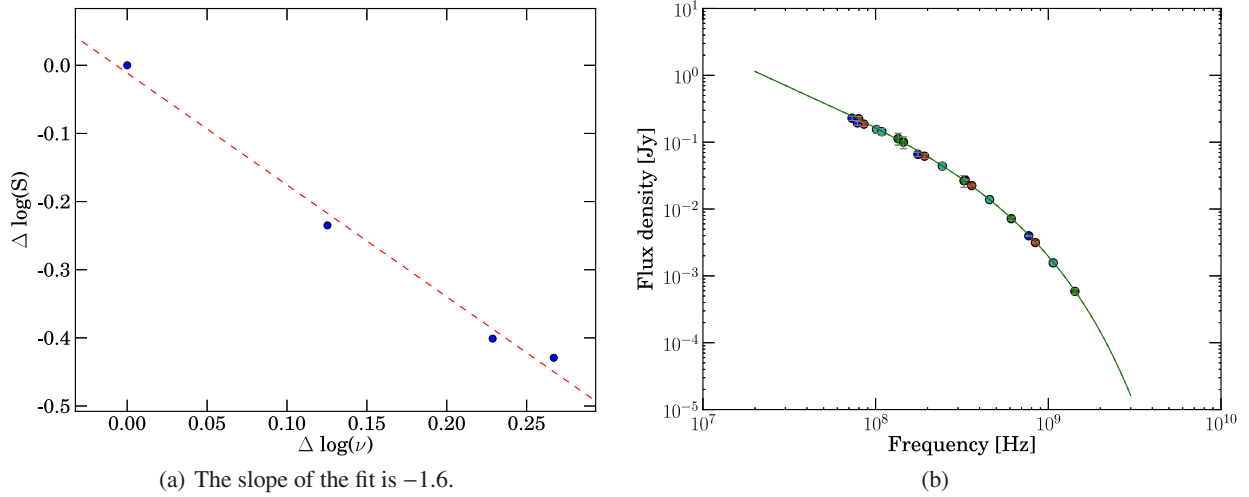
Fig. 6. Spectral shifts in \log(\nu) - \log(S) for Regions 3, 6, 9, and 10 in panel a). The dashed red line shows the best linear fit to the data points. Shifted data points giving the global spectrum are given in panel b). Different colours are used to indicate the data points belonging to different regions. The best JP and KGJP model fits are plotted with dashed-dot red and green lines, respectively (overlapping, since there is essentially no difference between the models for these regions).
