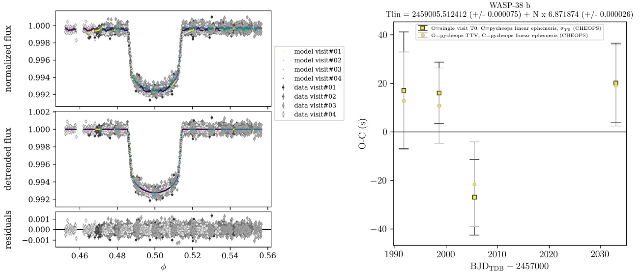
Figure 7. As in Fig. 2, but for WASP-38 b. Left: multivisit phase plot of four CHEOPS visits; right: O - C diagram.
