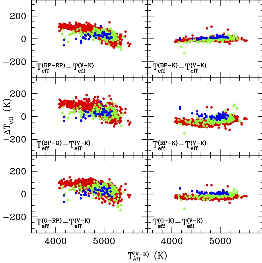
Fig. 2. Differences between T_{\text{eff}} derived from the Gaia colours and from (V - K_s)_0 as a function of the (V - K_s)_0 -based T_{\text{eff}} for the giant stars in three Galactic globular clusters, namely NGC 7099 (blue points), NGC 6752 (green points) and NGC 104 (red points).
