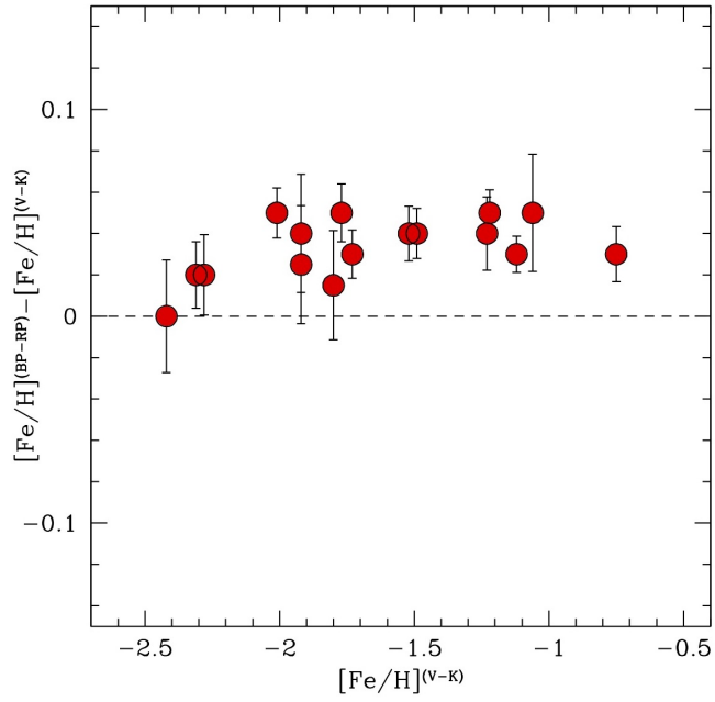
Fig. 4. Behaviour of (V-K)_0 and (BP-RP)_0 based [\text{Fe}/\text{H}] as a function of the iron content [\text{Fe}/\text{H}] derived from (V-K)_0 based T_{\text{eff}} for the 16 Galactic globular clusters analysed in Mucciarelli & Bonifacio (2020).
