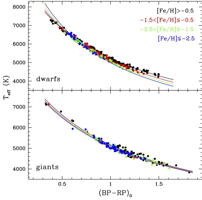
Fig. A.1. Behaviour of T_{\text{eff}} derived from IRFM by González Hernández & Bonifacio (2009) as a function of the (BP - RP)_0 colour, for dwarf and giant stars (upper and lower panels, respectively). The stars are grouped according to their metallicity: [Fe/H] \leq -2.5 dex (blue points), -2.5 < [Fe/H] \leq -1.5 (green points), -1.5 < [Fe/H] \leq -0.5 (red points), [Fe/H] > -0.5 dex (black points). The solid lines are the theoretical colour- T_{\text{eff}} relation calculated with [Fe/H] = -3.0 dex (blue line), -2.0 dex (red line), -1.0 dex (red line), +0.0 dex (black line).
