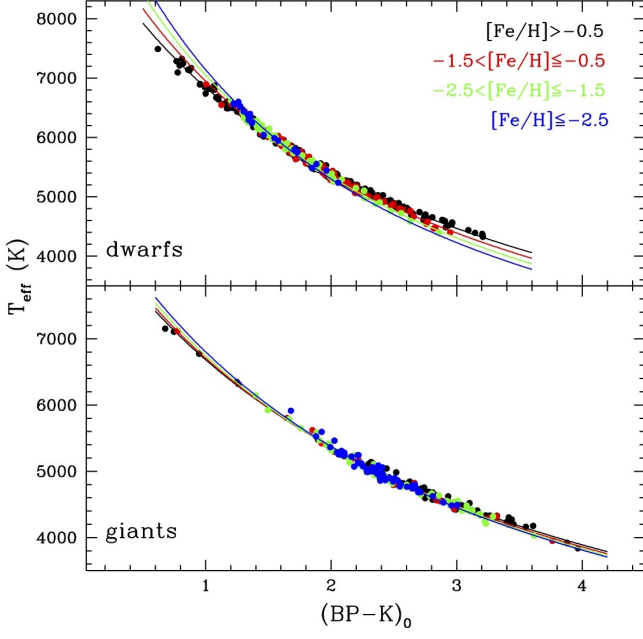
Fig. A.5. Same of Fig. A.1 but for the (BP - K_s)_0 colour.
