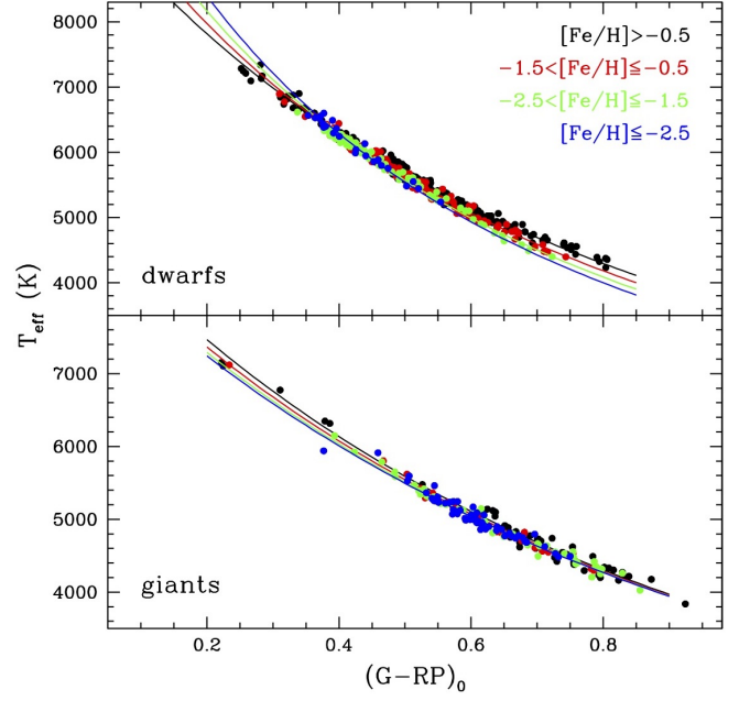
Fig. A.3. Same of Fig. A.1 but for the (G - RP)_0 colour.
