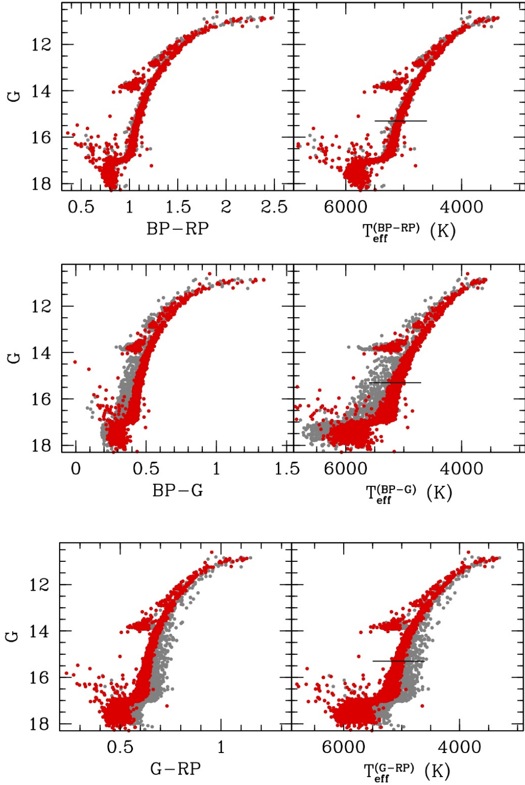
Fig. 3. Colour-magnitude diagrams for NGC 104 considering the pure Gaia colours (left panels) and the corresponding T_{\text{eff}} vs G-band magnitudes diagrams (right panels). Red and grey points mark the stars selected and rejected according to the criterion provided by R20, respectively. The horizontal lines in the right panels mark the transition between the dwarf and giant stars regimes.
