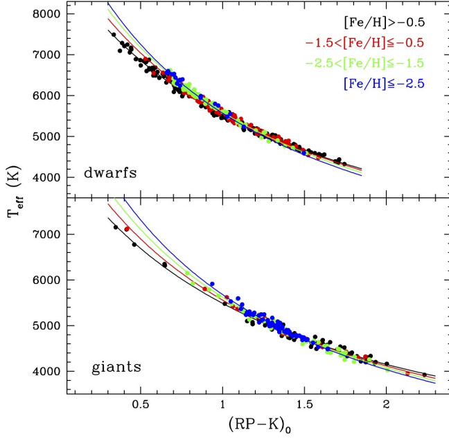
Fig. A.6. Same of Fig. A.1 but for the (RP - K_s)_0 colour.
