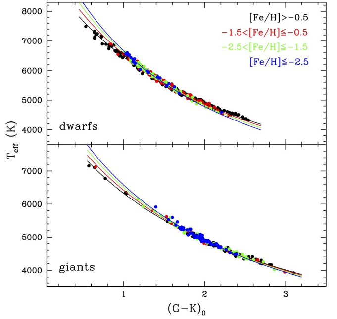
Fig. A.4. Same of Fig. A.1 but for the (G - K_s)_0 colour.
