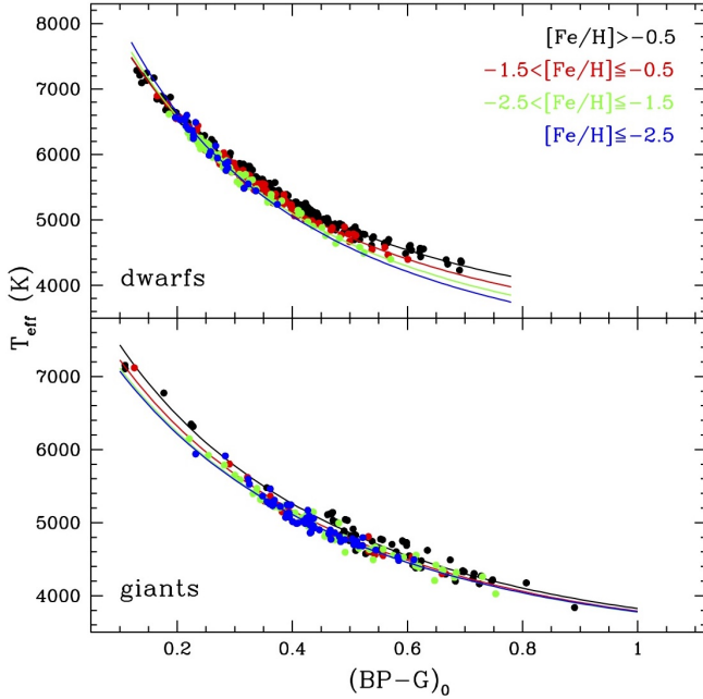
Fig. A.2. Same of Fig. A.1 but for the (BP - G)_0 colour.
