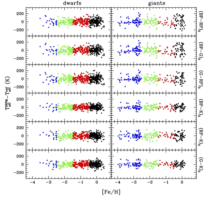
Fig. A.7. Behaviour of the temperature residuals as a function of [Fe/H] for all the colour- T_{\text{eff}} transformations discussed in this work. Colours are the same of previous figures.
