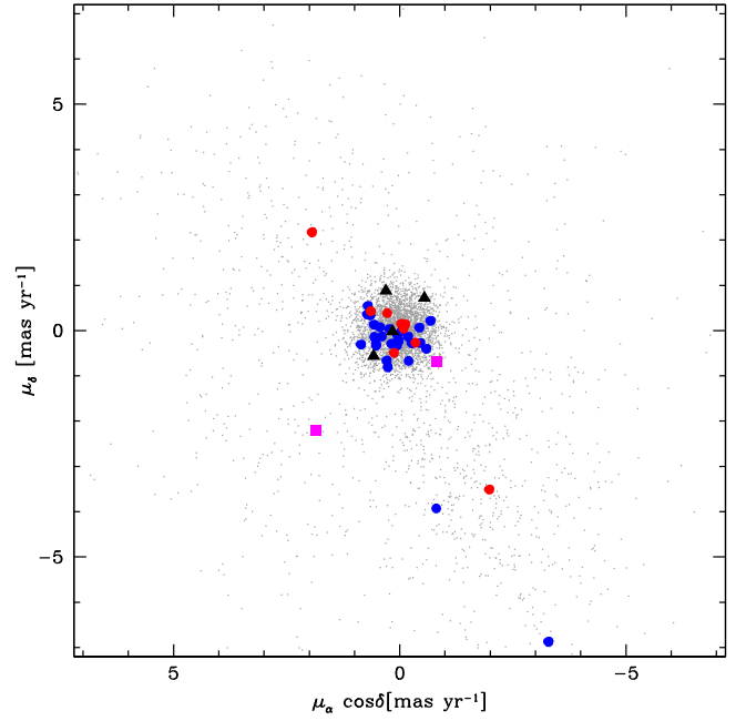
Figure 11. VPD for the spectroscopic targets discussed in Massari et al. (2014b) in common with our PM catalog. Blue circles are stars with -0.6 \leq [\text{Fe}/\text{H}] < 0 , and red circles have 0 \leq [\text{Fe}/\text{H}] < 0.5 . These represent the two main populations of Terzan 5. Black filled triangles correspond to stars belonging to the newly discovered third, metal-poor population. All three components are clearly genuine members of the system, being located well within the PM distribution of the cluster members. The two magenta filled squares represent the super-metal-rich stars of the spectroscopic sample, and, at odds with the other sources, they seem not to belong to Terzan 5.
