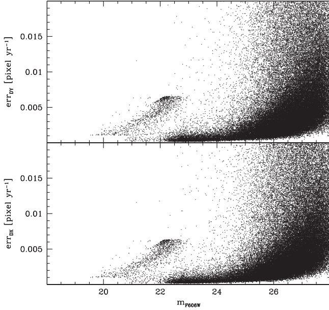
Figure 2. Uncertainties in the X and Y displacements in units of \text{pixel yr}^{-1} . Bright, well-measured stars have displacement errors typically smaller than 0.007 \text{ pixel yr}^{-1} in each coordinate. The separated sequence at larger errors that arises for m_{\text{F606W}} < 22.5 is made up of stars measured only in the short exposures.
