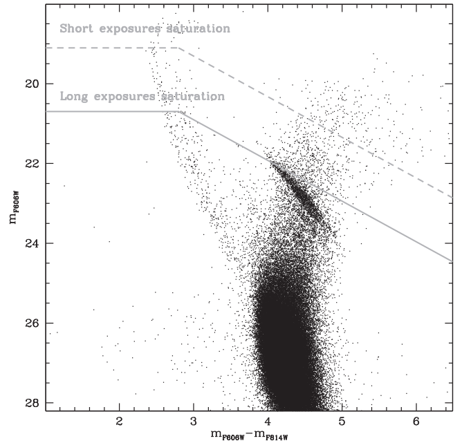
Figure 1. The (m_{F606W}, m_{F606W} - m_{F814W}) CMD of Terzan 5. All of the cluster evolutionary sequences are broadened because of the differential reddening effect. A bright, blue sequence is clearly separated from the cluster sequences, and it is likely composed of young field stars. The magnitude saturation limits of the short and long exposures are marked with the dashed and solid lines, respectively.
