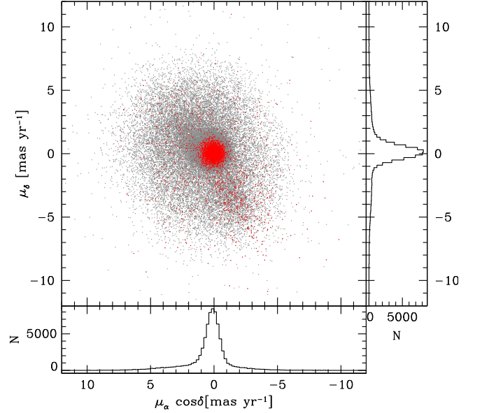
Figure 3. Vector point diagram (VPD) of the PMs measured for 70,324 stars (black dots) in the direction of Terzan 5. Their distribution in the R.A. and decl. PM-component axes is shown in the histograms in the bottom and right panels, respectively. PMs measured for unsaturated stars with m_{\text{F606W}} < 24 mag are shown as red dots. At least two components are visible: the first showing a symmetric distribution centered around the origin and an asymmetric structure roughly centered at (-1.8, -3.5) \text{ mas yr}^{-1} .
