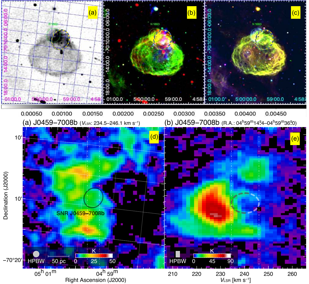
Figure A5. J0459 – 7008b: same as Fig. A1. Gray scale at the bottom of panel A (ASKAP image) is from 0 to 5 mJy beam -1 .
