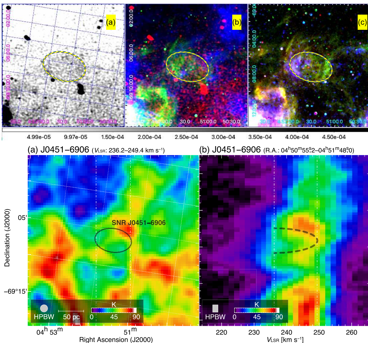
Figure A1. J0451 – 6906: (top panel) left-hand panel (A): New ASKAP 888-MHz radio image at a spatial resolution of 13.9 \times 12.1 arcsec 2 and PA -84^\circ . Gray scale at the bottom is from 0 to 0.5 mJy beam -1 . Middle panel (B): RGB image where ASKAP 888-MHz radio image is in red, H \alpha (green) and Spitzer LMC-SAGE at 8 \mu m in blue. Right-hand panel (C): MCELS optical RGB image where H \alpha (red), [S II] (green), & [O III] (blue). Bottom left-hand panel (D): integrated intensity map of H I obtained with ATCA and Parkes (Kim et al. 2003). The vertical dash-dotted (white) lines indicate the RA integration range for the position–velocity diagram. The blue–yellow ellipse indicates positions of here proposed SNR. Right-hand panel (E): position–velocity diagram of H I. The dashed curve delineates a cavity-like structure of H I. The vertical dash-dotted lines indicate the velocity integration range for the H I integrated intensity map.
