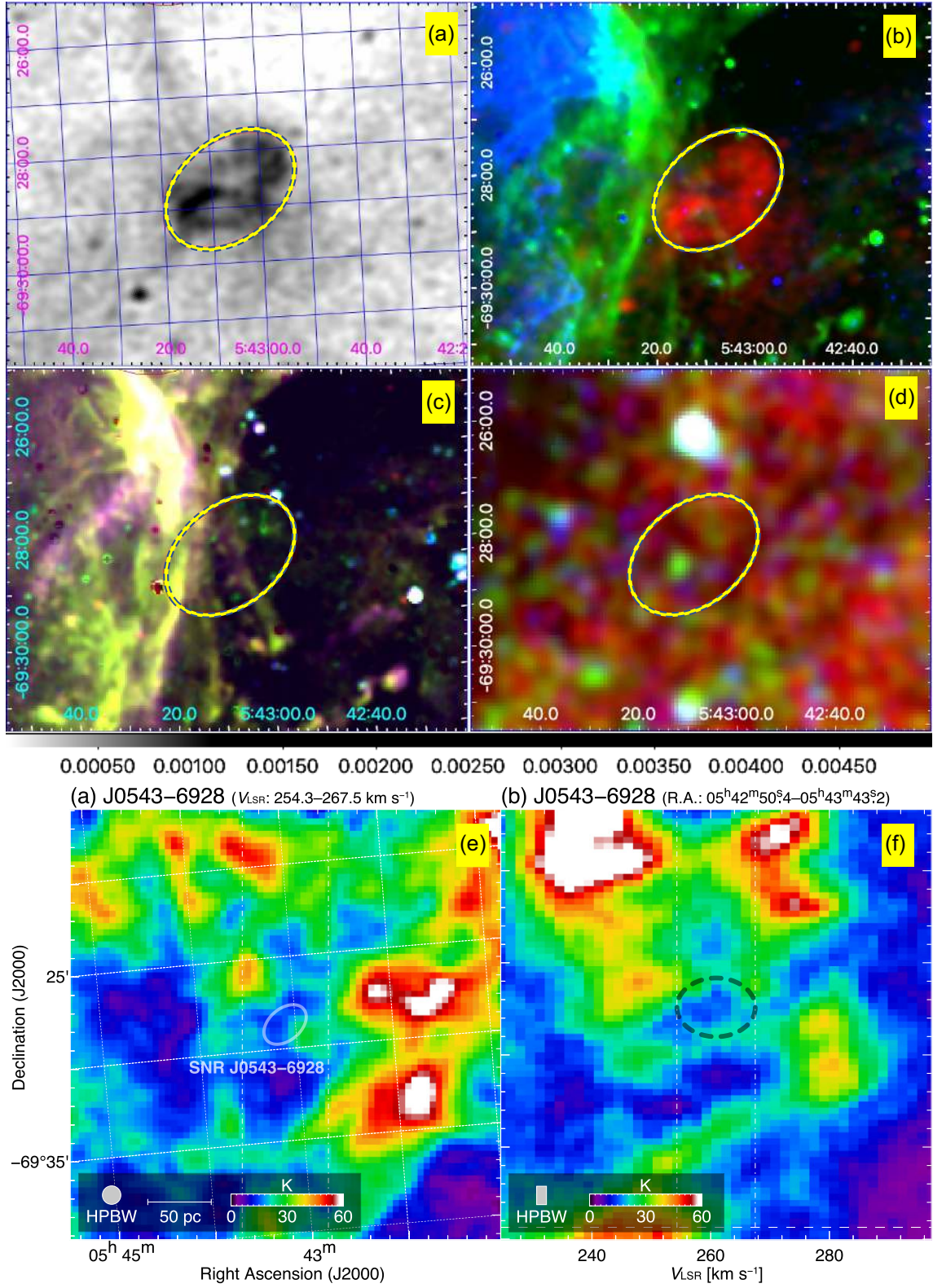
Figure A13. J0543 – 6928: same as Fig. A2. Gray scale at the bottom of Panel A (ASKAP image) is from 0 to 5 \text{mJy beam}^{-1} .
