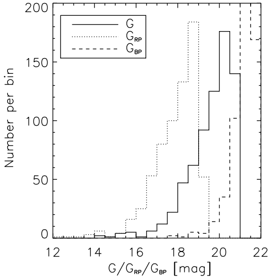
Figure 1. Top: distribution of optical and infrared spectral types in the GUCDS. Optical L0 and L1 bins have been truncated (they contain 202 and 105 objects, respectively). Bottom: distribution of Gaia magnitudes in the GUCDS.
