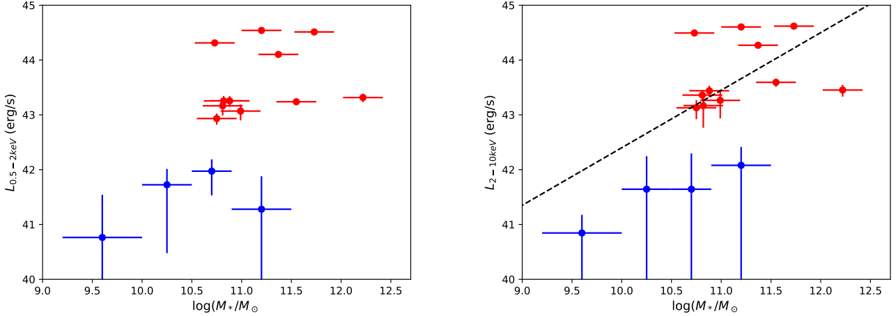
Fig. D.1. Left panel: the red points show the distribution of 12 protocluster members (including the Spiderweb Galaxy but excluding the two Compton-thick candidates) in the soft-band, intrinsic luminosity and stellar mass plane. Blue points are obtained stacking the protocluster members without X-ray detection in bins of stellar mass. Note that stacked L_X values should be considered upper limits, since, despite the formal positive detection, all the stacked values are consistent with noise within 1 or 1.5 \sigma . Right panel: same as the left panel but in the rest-frame hard band.
