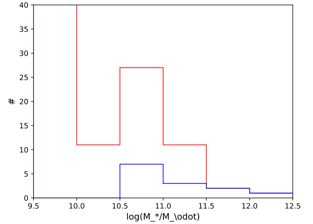
Fig. 21. Distribution of M_* among the protocluster members in the redshift range 2.11 < z < 2.20 (red histogram) and among the X-ray emitting members (blue histogram). The first bin ( 9.5 < \log(M_*) < 10.0 ) is actually an upper limit where we include all the sources that do not have K_S band counterpart in our image.
