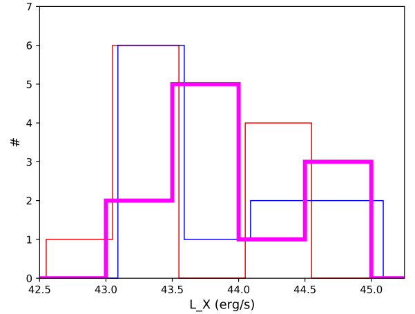
Fig. 15. The distribution of the X-ray luminosity of the 11 protocluster members (excluding the Spiderweb and the two Compton-thick candidates) in the soft (thin red line), hard (thin blue line) and total band (thick magenta line). For clarity, the histograms for the soft and hard luminosities are shifted by 0.05 and 0.1 dex, respectively.
