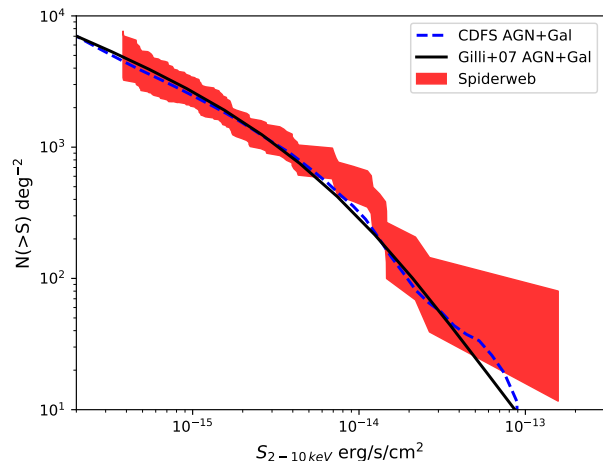
Fig. 6. Cumulative number counts in the hard band in the Spiderweb field, within 5 arcmin from the Spiderweb Galaxy (red shaded area). The shaded area shows the uncertainty due to the combination of source statistics, photometric errors and systematic uncertainty on the conversion factors. The blue, dashed line shows the hard counts in the CDFS from Luo et al. (2017). The black solid line shows the prediction from the AGN model of Gilli et al. (2007) plus the contribution from normal galaxies from Luo et al. (2017).
