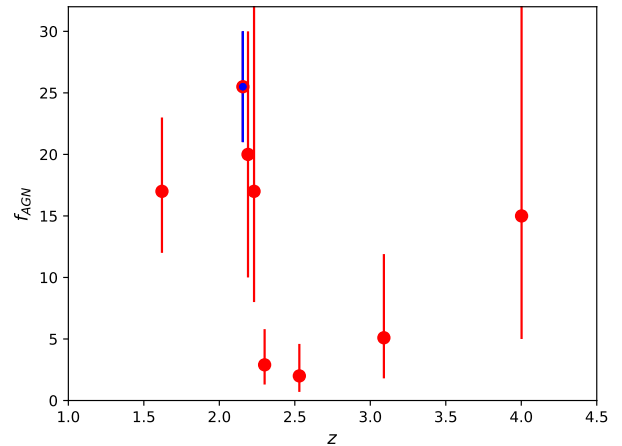
Fig. 22. The fraction of X-ray AGN over the total number of identified protocluster members from Table 6. The Spiderweb Protocluster is marked with a blue dot. The plot is meant to show the measurements of AGN fraction available in the literature, and, necessarily, includes measurements for different populations and different stellar mass ranges.
