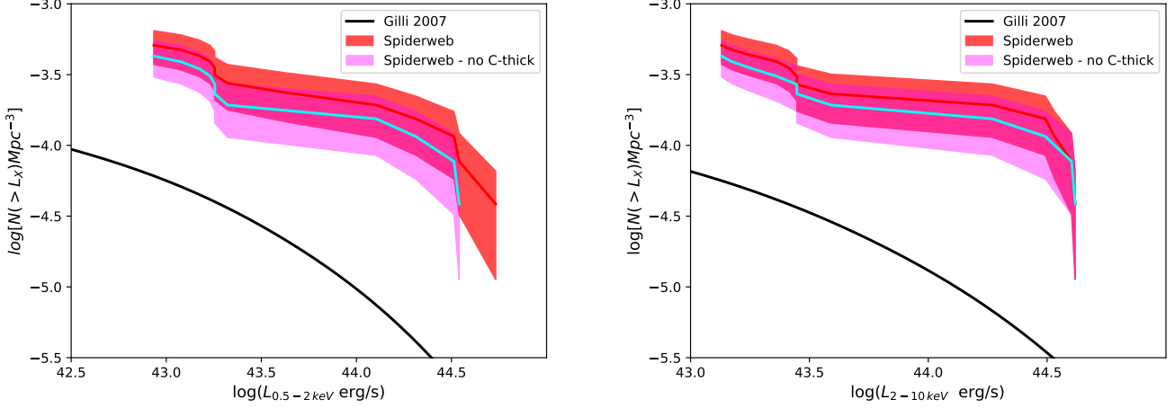
Fig. 19. Left panel: the red, solid line with the red-shadowed area shows the cumulative rest-frame, soft-band luminosity function of the AGN in the Spiderweb protocluster, normalized to the comoving volume defined by 2.11 < z < 2.20 and a circle of 5 arcmin centered on the Spiderweb Galaxy. The cyan solid line with the pink-shadowed area is the same without the luminosity correction for the two C-thick candidates. The black solid line is the XLF in the field from the model of Gilli et al. (2007) . Shaded areas correspond to 1\sigma uncertainty. The Spiderweb Galaxy is not included in the luminosity function. Right panel: same as left panel in the rest-frame, 2-10 keV hard band.
