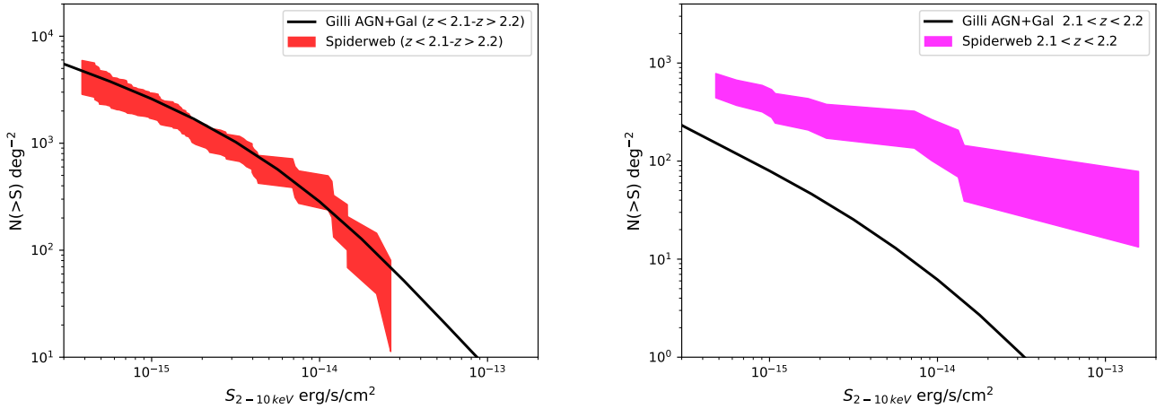
Fig. 12. Left panel: the hard band logNlogS in the Spiderweb field (within a radius of 5 arcmin) after excluding the X-ray sources identified in the 2.11 < z < 2.20 range, compared to the expectations from the model of Gilli et al. (2007) in the same redshift range. The shaded area corresponds to an uncertainty of 1\sigma . Right panel: the hard band logNlogS in the Spiderweb field only for the redshift interval 2.11 < z < 2.20 , compared to the expectations from the model of Gilli et al. (2007) in the same redshift range. The shaded area corresponds to an uncertainty of 1\sigma . Note the different scales between the two panels.
