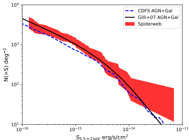
Fig. 5. Cumulative number counts in the soft band in the Spiderweb field, within 5 arcmin from the Spiderweb Galaxy (red shaded area). The shaded area shows the uncertainty due to the combination of source statistics, photometric errors and systematic uncertainty on the conversion factors. The blue, dashed line shows the soft counts in the CDFS from Luo et al. (2017). The black solid line shows the prediction from the AGN model of Gilli et al. (2007) plus the contribution from normal galaxies from Luo et al. (2017).
