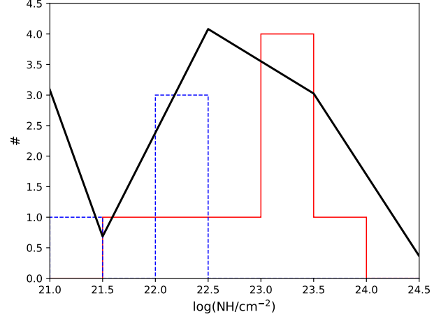
Fig. 14. The red histogram shows the distribution of the intrinsic absorption of the 8 protocluster members (including the Spiderweb) for which a robust measurement of N_H has been possible. The blue dashed histogram shows the upper limits on N_H obtained for 6 sources. The black solid line shows the distribution of N_H expected in the model of Gilli et al. (2007) at the flux limit of our observations. The two Compton-thick candidates, with a reflection-dominated spectrum, are not included.
