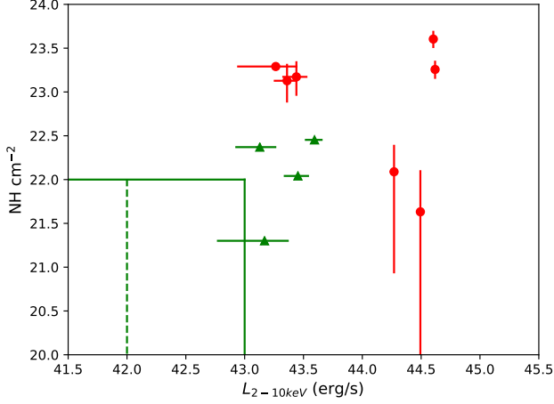
Fig. 16. Scatter plot of N_H and L_{2-10keV} for 11 sources (excluding the Spiderweb and the two Compton-thick candidates). Red circles correspond to measured N_H values, while green triangles to 1\sigma upper limits. The green box shows the parameter space still consistent with star formation at the level of 1000 M_\odot/\text{yr} or 100 M_\odot/\text{yr} (vertical dashed line).
