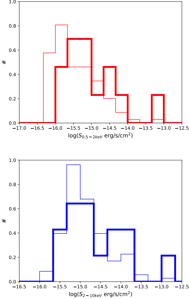
Fig. 13. Top panel: the differential, normalized distribution of the soft fluxes in the Spiderweb Galaxy Field. The total sample of X-ray sources is shown with a thin line, while the subsample of the 14 protocluster members are shown with a thick line. Bottom panel: same as in the top panel in the hard band.
