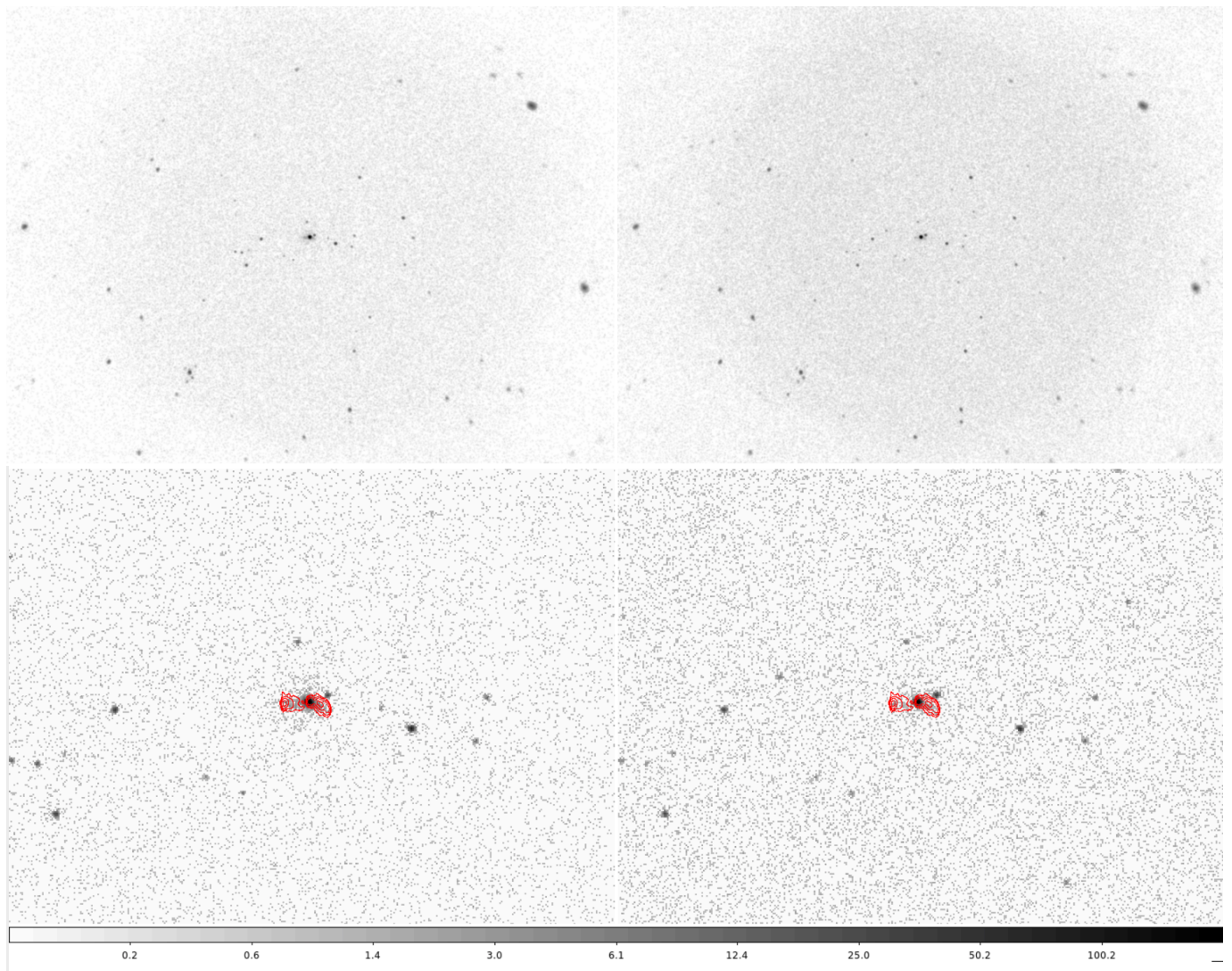
Fig. 3. Upper panels: Chandra X-ray images of the Spiderweb Galaxy field in the soft 0.5-2 keV (left) and hard 2-7 keV band (right). A box of 12 \times 9 arcmin by side centered on J1140-2629 is shown. The images have been smoothed with a \sim 1 arcsec Gaussian kernel to emphasize the unresolved sources. Sources at the outskirts of the image appear larger due to the effect of the increase of the PSF. Lower panels: close-up of the Spiderweb Galaxy ( 3 \times 2 arcmin by side) at full angular resolution, in the soft (0.5-2 keV, left) and hard (2-7 keV, right) band. Extended emission is clearly visible in both bands. Red contours show radio emission observed in the 10 GHz band with the JVLA (see Carilli & Anderson 2022) at levels of 0.03, 0.2, 2 and 20 mJy/beam.
