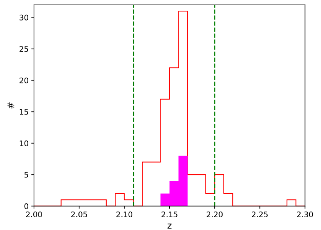
Fig. 10. Redshift distribution of the X-ray sources identified as protocluster members, including the one without spectroscopic confirmation (magenta filled histogram) compared to the redshift distribution of all the sources in the field with spectroscopic redshift in the range 2.0 < z < 2.3 . The dashed, vertical lines correspond to the protocluster redshift range.
