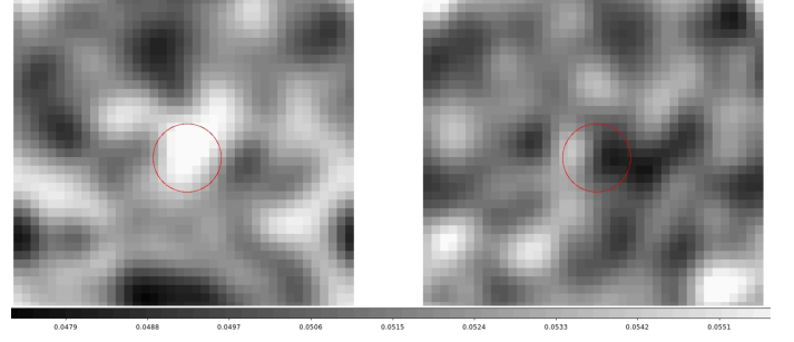
Fig. 18. Left panel: stacked image of the 81 color or narrow-band selected protocluster member candidates in the soft band. The red circle shows the 2 arcsec radius region used to perform aperture photometry on the stacked image. Right panel: same as in the left panel in the hard band.
