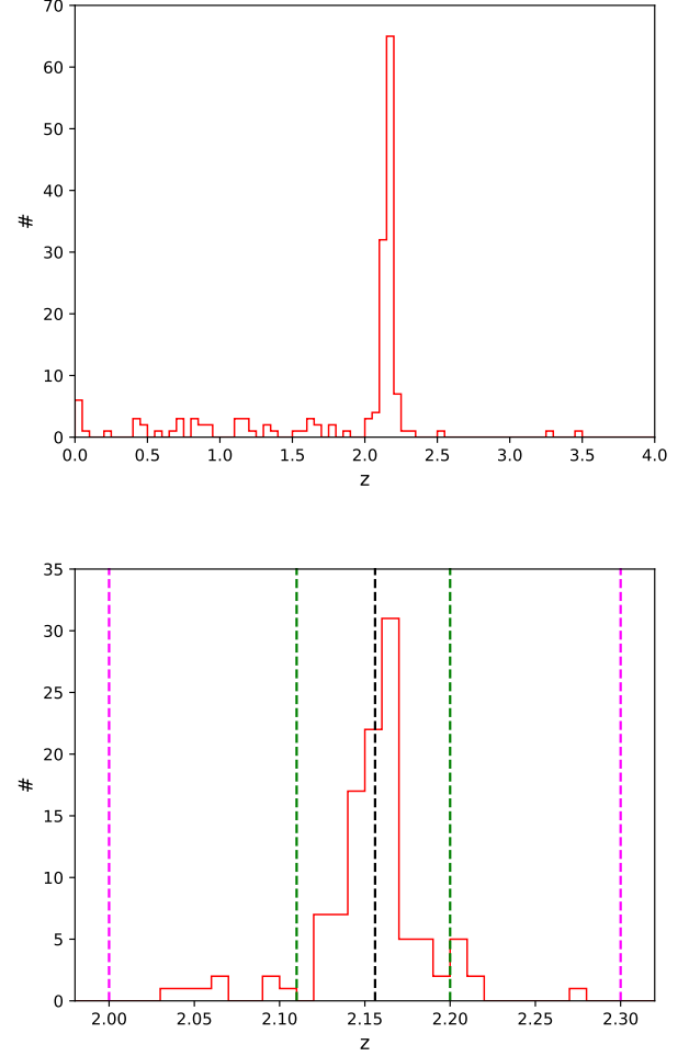
Fig. 1. Upper panel: Distribution of the 161 spectroscopic redshifts in the Spiderweb field. Lower panel: redshift distribution in the range 2.0 < z < 2.3 . Vertical dashed lines show the redshift of the Spiderweb Galaxy as measured with low resolution spectroscopy by van Ojik (1995) (black line), the range adopted to define the Spiderweb Complex (magenta lines) and the protocluster (green lines), as discussed in the text.
