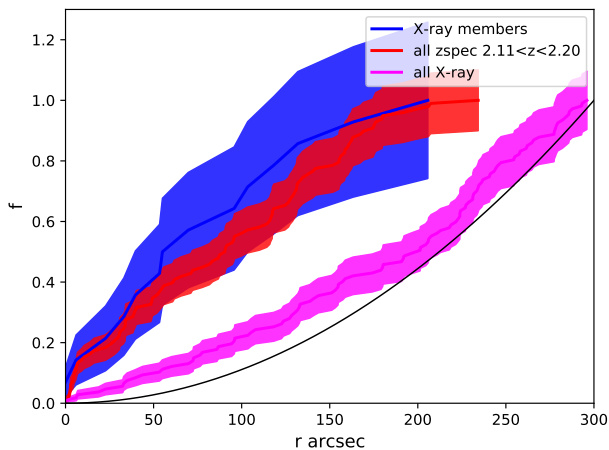
Fig. 9. The fraction of sources within a given radius from the Spiderweb Galaxy. X-ray cluster members (shown in blue) have the same distribution of all the spectroscopically-confirmed protocluster members in the 2.11 < z < 2.20 range (shown in red). On the other hand, the distribution of all the X-ray sources (dominated by the field) is clearly less clustered. The thin black line shows a perfectly uniform source distribution. The shaded area corresponds to an uncertainty of 1\sigma .
