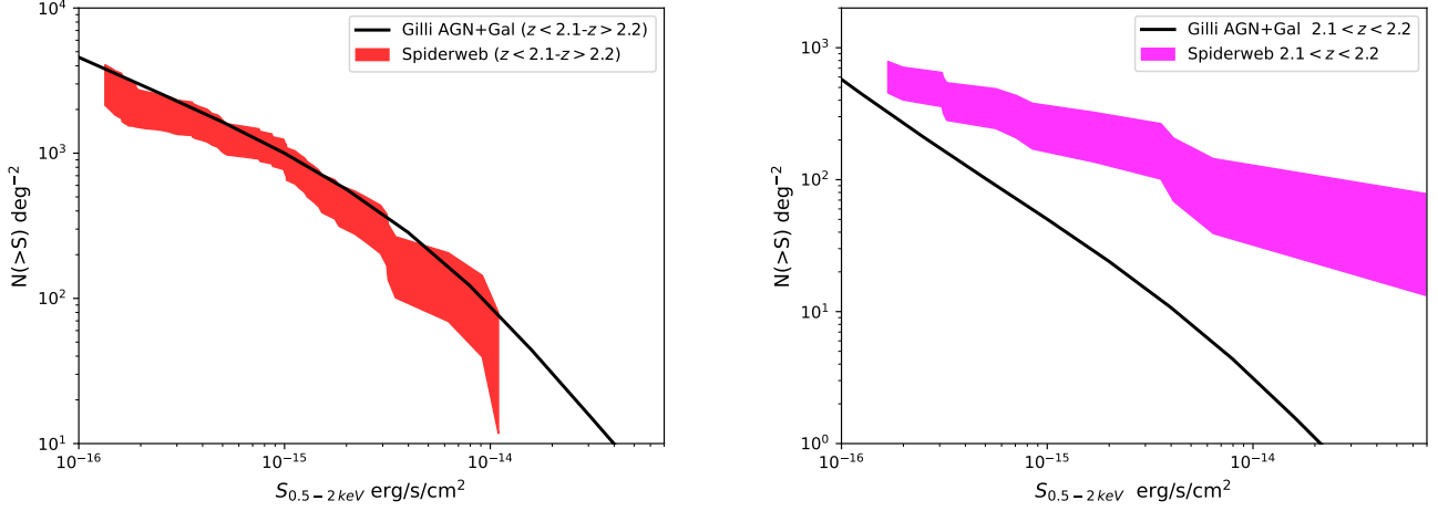
Fig. 11. Left panel: the soft band logNlogS in the Spiderweb field (within a radius of 5 arcmin) after excluding the X-ray sources identified in the 2.11 < z < 2.20 range, compared to the expectations from the model of Gilli et al. (2007) in the same redshift range. The shaded area corresponds to an uncertainty of 1\sigma . Right panel: the soft band logNlogS in the Spiderweb field only for the redshift interval 2.11 < z < 2.20 , compared to the expectations from the model of Gilli et al. (2007) in the same redshift range. The shaded area corresponds to an uncertainty of 1\sigma . Note the different scales between the two panels.
