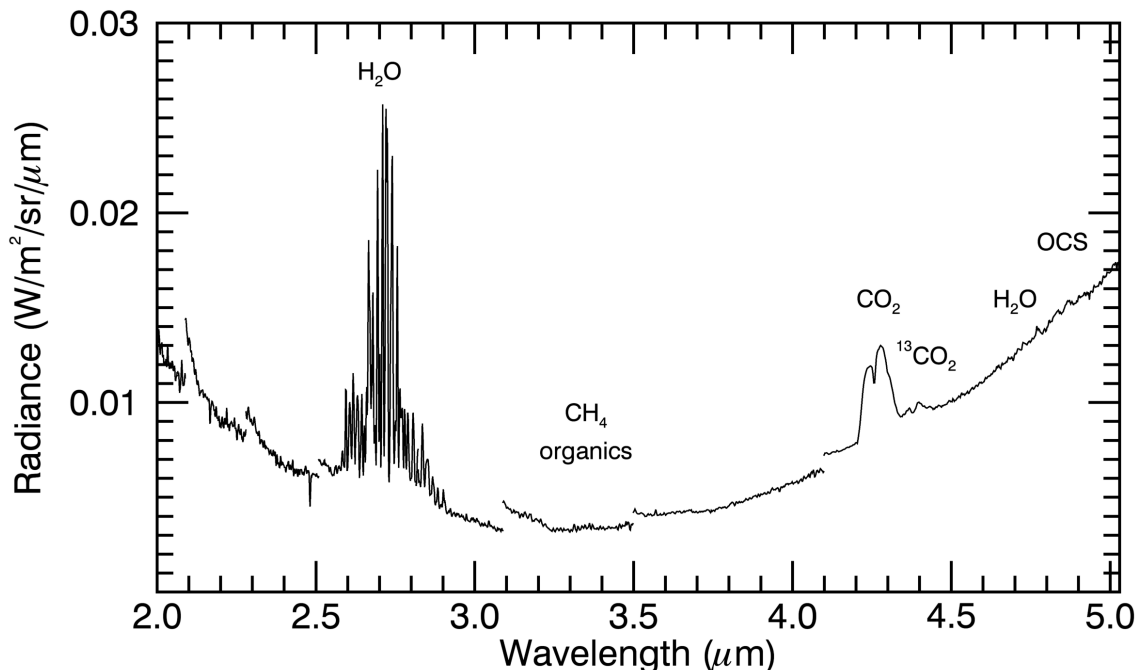
Figure 1. Full VIRTIS-H spectrum obtained by averaging the 3 data cubes obtained on 19 Aug. 2015. At this scale, the faint emissions from CH 4 , OCS and H 2 O 4.5–5 \mu m bands are not easily distinguishable. The short wavelength range of the spectral orders is contaminated by instrumental straylight (e.g., at 2.1 and 2.28 \mu m), resulting in a higher radiance.
