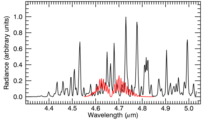
Figure 4. Simulated fluorescence spectra of \text{H}_2\text{O} (black) and \text{CO} (red) for an effective spectral resolution of 800. The \text{CO}/\text{H}_2\text{O} abundance ratio is 1% and the rotational temperature is 100 K.
