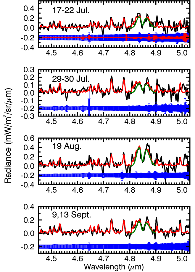
Figure 3. VIRTIS-H spectra in the range 4.45–5 \mu m showing ro-vibrational lines of the H 2 O \nu_3 - \nu_2 band, and the OCS \nu_3 band. The red line displays the fitted synthetic spectrum for a temperature of 120 K, including both H 2 O and OCS. The green line shows the contribution due to OCS only. A: 17–22 July; B: 29–30 July; C: 19 Aug.; D: 9, 13 Sept. The standard deviation for each spectral channel is shown in the bottom of the plots (for better reading, the errorbars are offsetted with respect to the measured radiances); values in blue include time variations in the continuum. In the top plot, the standard deviation measured on a spectrum with no comet signal (and scaled to the observing time of the comet spectrum) is superimposed, in red.
