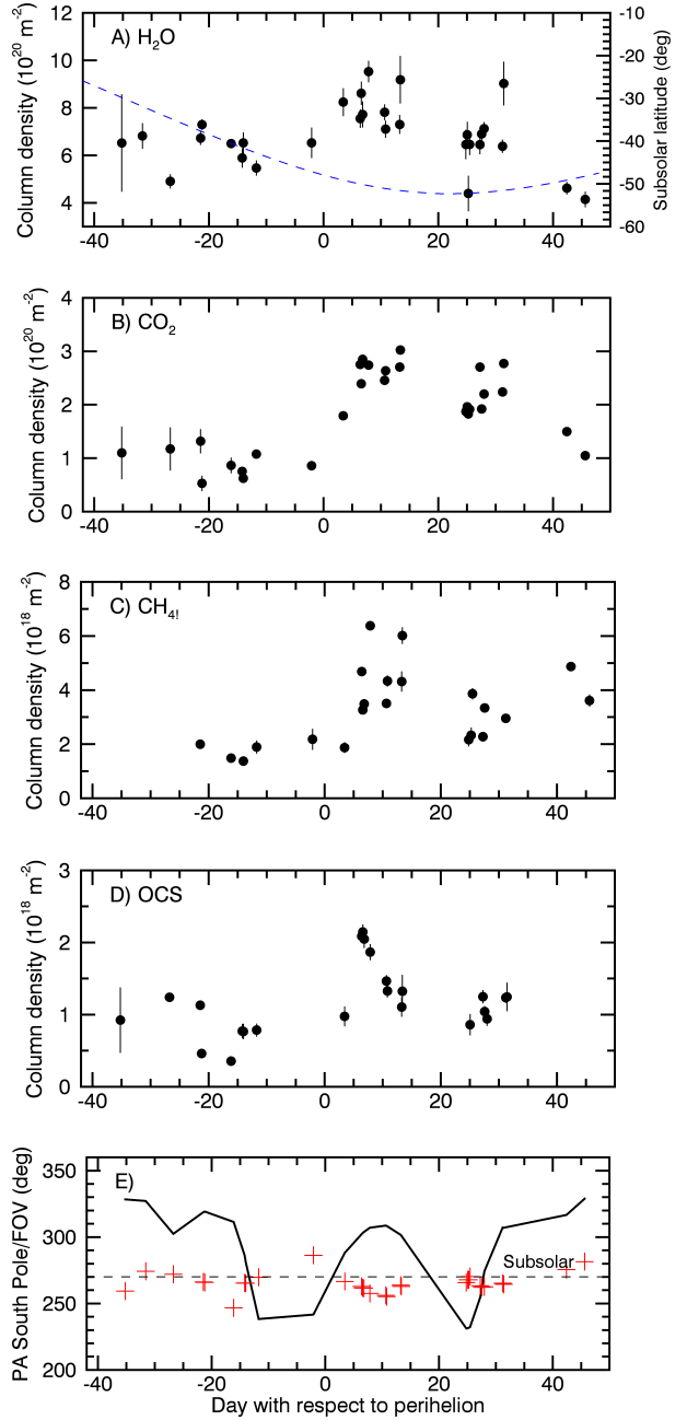
Figure 9. Column densities of \text{H}_2\text{O} , \text{CO}_2 , \text{CH}_4 and \text{OCS} as a function of date with respect to perihelion (A–D), and position angles of the South pole direction and FOV (E). A–D) Measured column densities (dots with error bar) are rescaled to a distance of \rho = 4 km assuming a 1/\rho variation; the latitude of the subsolar point is plotted as a dashed line in plot A. E) The PA of the South direction is shown as a black line; the PA of the FOV are plotted with crosses; the projected comet-Sun direction at PA = 270^\circ is indicated as a dashed line.
