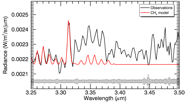
Figure 6. VIRTIS-H spectrum in order 2 covering the \text{CH}_4 \nu_3 band, obtained by averaging 9 data cubes showing well detected \text{CH}_4 emission ( \text{SNR} > 20 ). The synthetic spectrum of \text{CH}_4 computed for a rotational temperature of 100 K is shown in red. The standard deviations are shown in the bottom of the plot (see Fig. 3). Species other than \text{CH}_4 (in particular \text{C}_2\text{H}_6 and \text{CH}_3\text{OH} ) contribute to the signal longward 3.32 \mu\text{m} .
