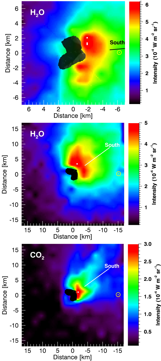
Figure 2. VIRTIS-H raster maps of the H 2 O 2.7 and CO 2 4.3 \mu m bands. Top: H 2 O on 30 July 2015, 19h:25 UT (ObsId: 00396898661). Middle and bottom: H 2 O and CO 2 , respectively, on 9 August 2015, 3h:10 UT (ObsId: 00397703949). The projection of the rotation axis (South direction) and Sun direction are indicated. The observational parameters are: line spacing of 0.6 km and 2 km, slew rate of 1.0 and 1.75 deg/min, for 30 July and 9 August, respectively. The maps were obtained after averaging spectra within cells of sizes of 1 km (30 July) and 2 km (9 August).
