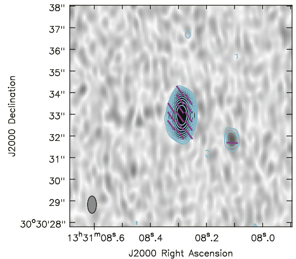
Figure 1. Cyan contours show Stokes I intensity, grayscale shows polarized intensity ( \sqrt{Q^2 + U^2} ), and magenta vectors show the polarization position angle of 3C 286. The contours are plotted at (-1, 1, 2, 4, 8, 16, 32, 64, 128, 512) \times 0.15 \text{ mJy beam}^{-1} , which is 3\times the rms noise in the Stokes I image. The EVPA is plotted at levels >3\sigma \times the rms noise in the polarized intensity map. The restoring beam is 0''.797 \times 0''.406 at a position angle of -180^\circ , which is given by the ellipse at the bottom left corner of the image.
