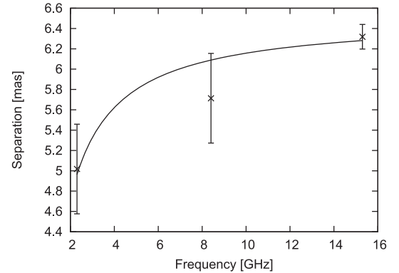
Figure 5. The separations between C1 (core) and C2 as a function of frequency. The curved line is the best-fit power law: r_c = (6.51 \pm 0.17) + (-3.57 \pm 1.13)\nu^{-1} .
