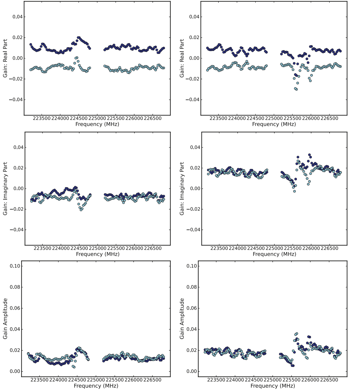
Figure 6. Examples of D -terms. The left and right columns show the D -term spectra for antennas DA41 and DV01, respectively. The upper, middle, and lower panels show the real part, imaginary part, and amplitude of the D -terms. Blue and cyan symbols represent D_X and D_Y . Note that the D -terms presented in this figure were not computed in the telescope frame but in the sky frame; this solution can be obtained using the CASA command dxy in almapolhelpers.py .
