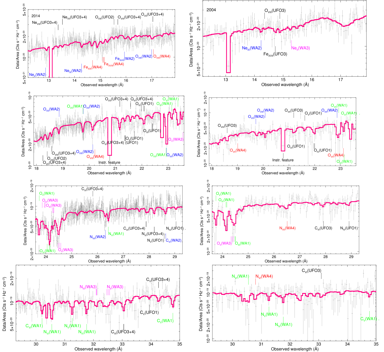
Figure 1. Detector area-corrected data and best-fitting model with a Galactic-absorbed continuum (4 WAs + 4 2) UFOs applied to the 2014 (2004) spectrum on the left-hand (right-hand) panels. We show the entire broadband in four wavelength ranges, from top to bottom: 12.2–17.9 Å, 17.9–23.6 Å, 23.6–29.3 Å, and 29.3–35 Å. The main absorption lines produced by every component are plotted in different colors: WA 1 in green, WA 2 in blue, WA 3 in magenta, WA 4 in red, and the UFOs in black. Every line marked in this figure is included in Table 2.
