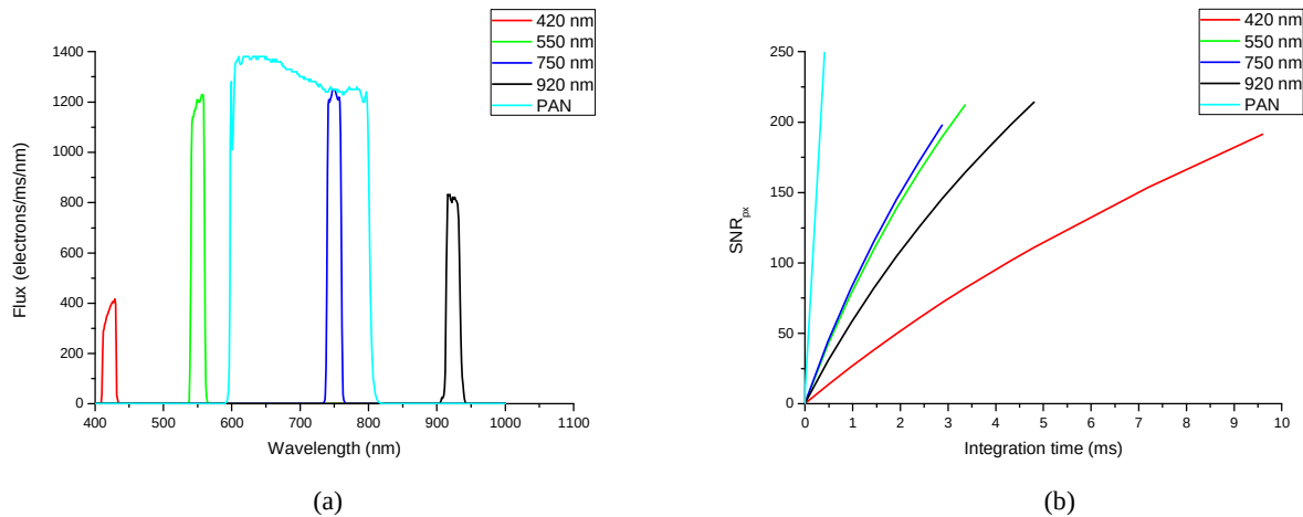
Figure 10. (a) Expected spectral flux in electrons/ms/nm and (b) calculated SNR versus integration time for each filter for the case Mercury at aphelion S/C at perihelion.
