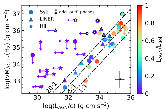
Figure 19. Relation between outflow momentum rate ( v_{\text{outf}} \dot{M}_{\text{outf}} ) and AGN radiative momentum rate ( L_{\text{AGN}}/c ). The theoretical predictions ( v_{\text{outf}} \dot{M}_{\text{outf}}/L_{\text{AGN}}/c \sim 20:1 (energy driven) and 1:1 (momentum driven) are shown as a dashed lines, respectively. Radiation pressure-driven outflows can reach ( v_{\text{outf}} \dot{M}_{\text{outf}}/L_{\text{AGN}}/c \sim 5:1 ). Colour-coding and symbols are same as in Fig. 2.
