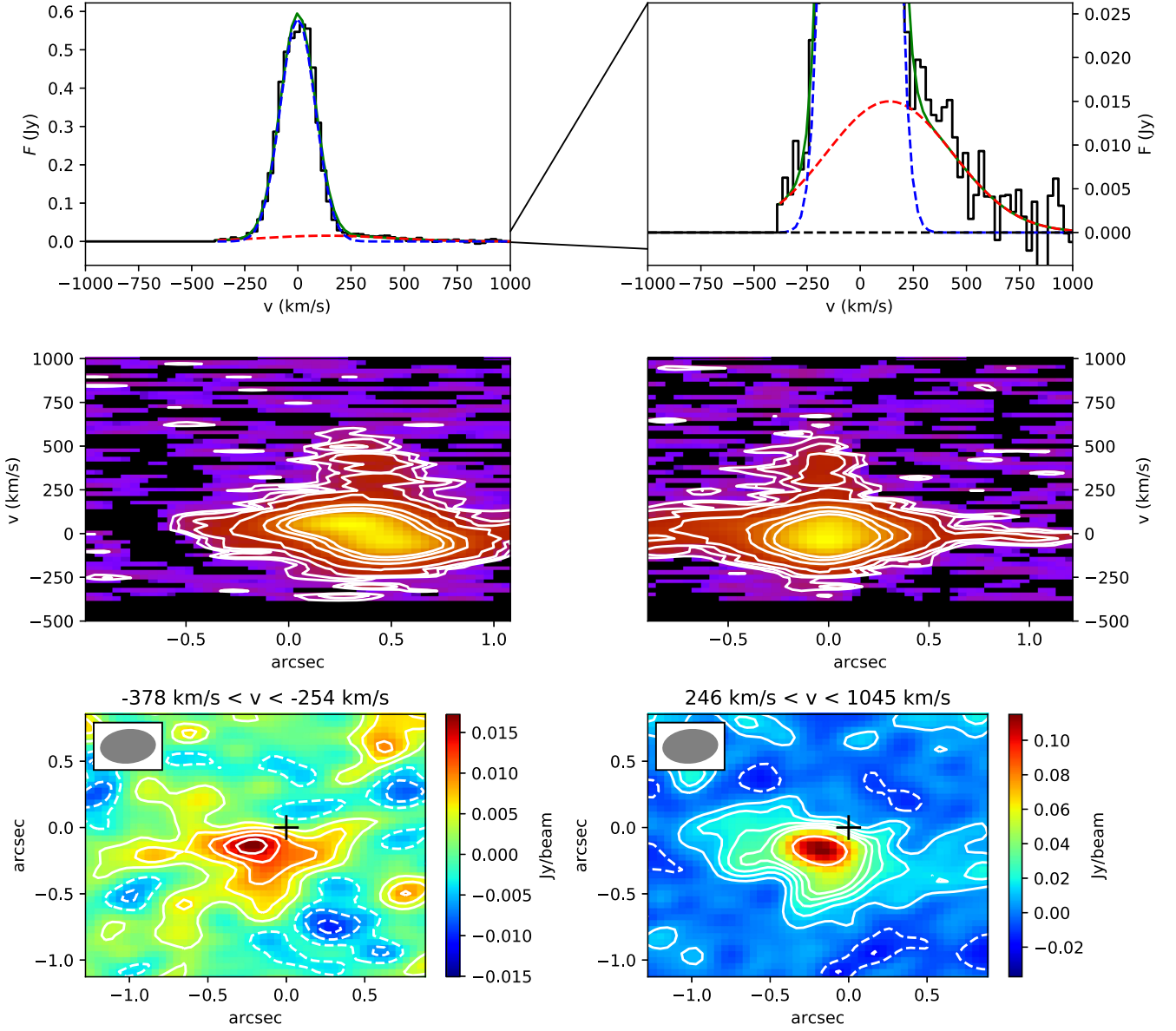
Figure A2. IRAS 05189 – 2524: see caption of Fig. A1, but contours in p - v diagrams (middle panel) are (2, 3, 5, 10, 30, 50, 70) \sigma .
