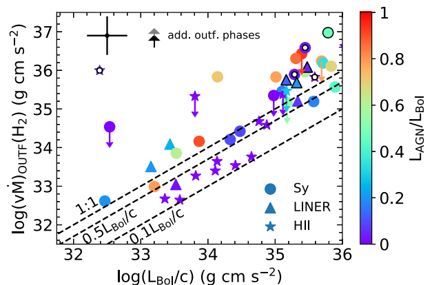
Figure 20. Dependence of the outflow momentum rate ( v_{\text{outf}} \dot{M}_{\text{outf}} ) on the total photon momentum output of the galaxy (i.e. from AGN and star formation). The top dashed line indicates the 1:1 relation between momentum rate and bolometric luminosity, while lower dashed lines indicate lower ratios. Colour-coding and symbols are same as in Fig. 2.
