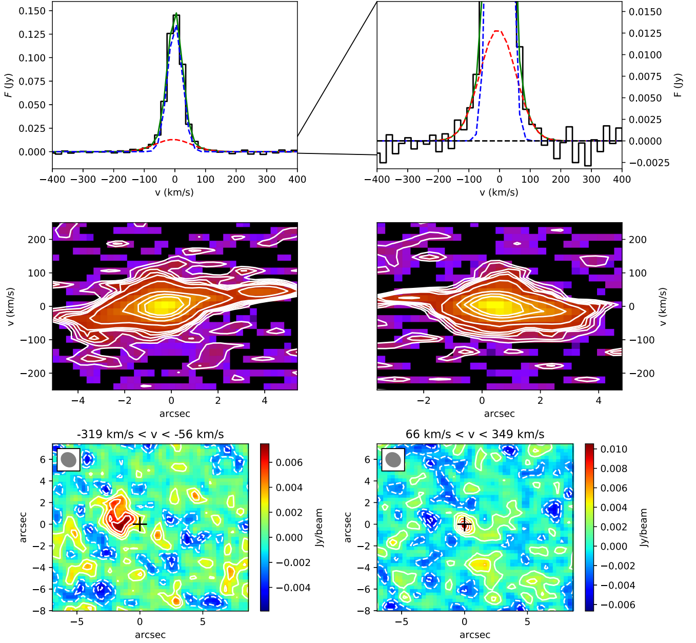
Figure A6. IRAS15515 + 0208: see caption of Fig. A1.
