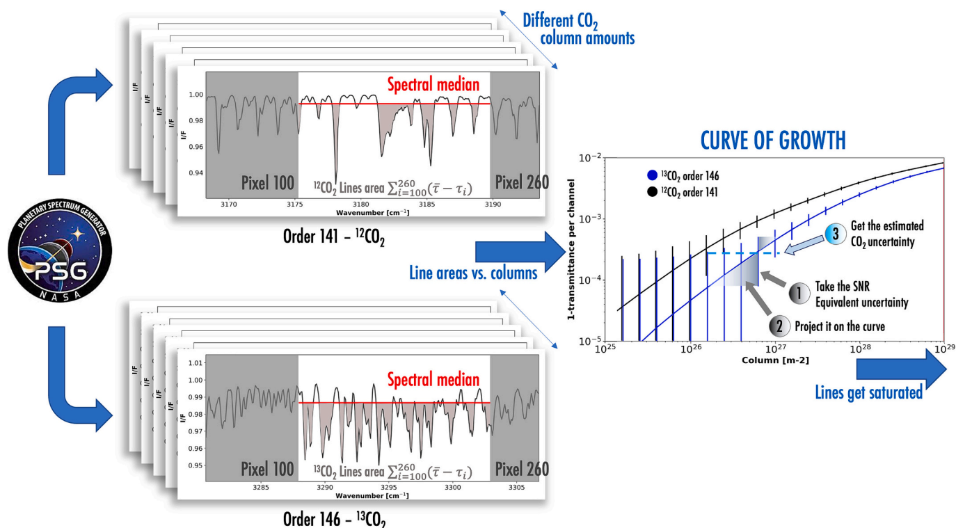
Fig. 7. Illustration of the SPEX method to get a quantitative estimation of the best achievable uncertainty on CO 2 retrievals based on the curve of growth and radiometric noise.
