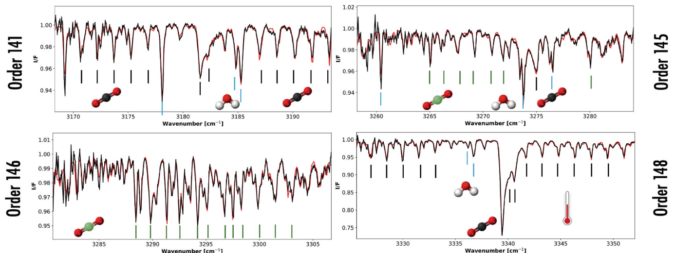
Fig. 2. Sample spectra acquired by NOMAD during a fullscan at the same altitude ( \sim 25 km) at L_S 171 MY34 (May 7, 2018, 17:27 UTC). For each order, lines from water vapor (light blue), ^{12}\text{CO}_2 (black) and ^{13}\text{CO}_2 (green) are marked. It is also highlighted that order 148 is used to get a sensitive measurement of the atmospheric temperature. Observations are the continuous black line, and the best fit is in red, to showcase the typical modeling accuracy. Spectra are shown in I/F units, i.e., in Solar Occultation geometry, the atmospheric transmittance along the line of sight. (For interpretation of the references to color in this figure legend, the reader is referred to the web version of this article.)
