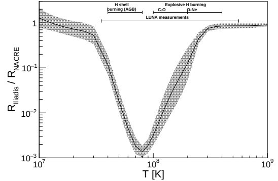
Figure 9: Ratio between the thermonuclear reaction rate calculated by Ref. [77] and NACRE [8].
