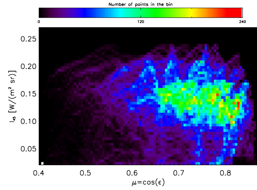
Fig. 7. Data points from Fig. 6, once binned in the (I_{45}, \mu=\cos(\epsilon)) space. Bins have widths of 0.005 W/(m^2 sr) and 0.005 (dimensionless) in the two directions. a. Mean value of JIRAM signal ( I ) inside each bin, b. Standard deviation of I inside each bin (note the different scale with respect to panel a.), c. Number of data points (triplets) inside each bin.
