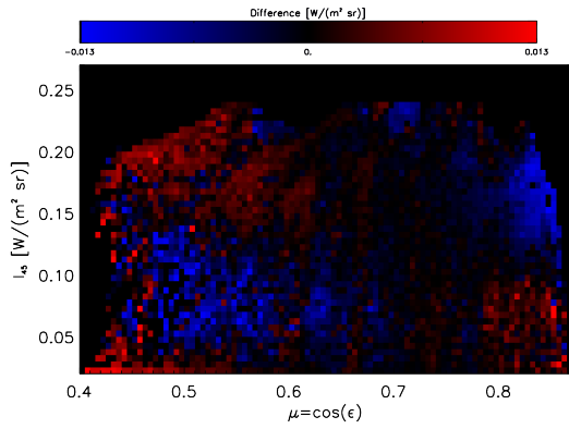
Fig. 9. a. Simulated I = f_{\text{simul}}(I_{45}, \epsilon) for \omega_0 = 0.90 and g = 0.37 , best-fit values inferred from Fig. 8 b. Difference between experimental data and the best-fit surface (i.e.: between Fig. 7a and Fig. 9a.) c. Ratio between fit discrepancies (Fig. 9a) and spread of experimental data (Fig. 7b).
