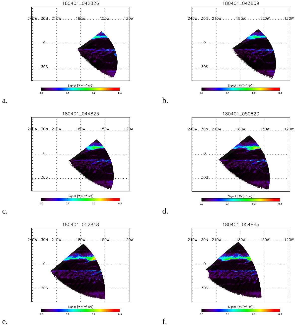
Fig. 1 Mosaics of JIRAM M-band images acquired during the 12 th Juno perijove passage. Each mosaic is derived from a single JIRAM sequence (see text for a definition). The title of each panel provides the central acquisition time according the scheme yymmdd_hhmmss. Note the progressive signal increase at (7^\circ\text{N}, 162^\circ\text{W}) in panels a.-e. caused by decreasing emission angles (see Table I for further details). Cylindrical projection is adopted.
