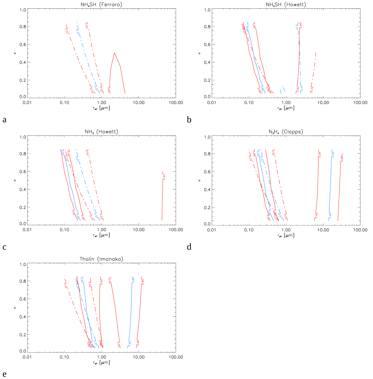
Fig. 10. Contour lines for \omega_0 (solid curves) and g (dashed curves) in the r_{\text{eff}} – variance space. Blue curves gives the values estimated from JIRAM data, red curves the acceptance region bounded by corresponding uncertainties as estimated from Fig. 6. a. \text{NH}_4\text{SH} , with complex refractive indices from Ferraro et al. b. \text{NH}_4\text{SH} , from Howett et al. c. \text{NH}_3 , from Howett et al. d. \text{N}_2\text{H}_4 , from Clapp and Miller, e. tholin type 2 from Imanaka et al.
