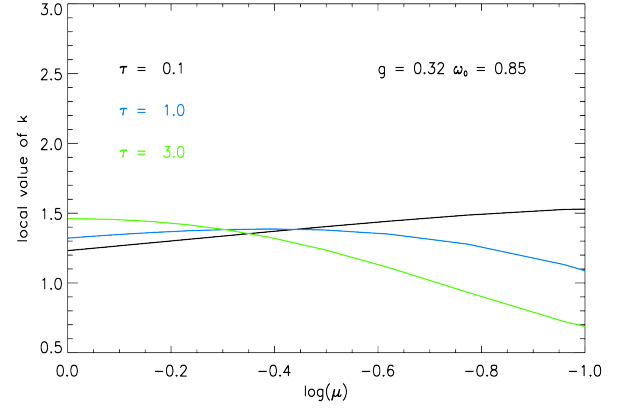
Fig. 3 Examples of k values for Minnaret functions modeling theoretical limb darkening in typical Hot-Spot conditions. The parameter depends both on \mu as well as on \tau .
