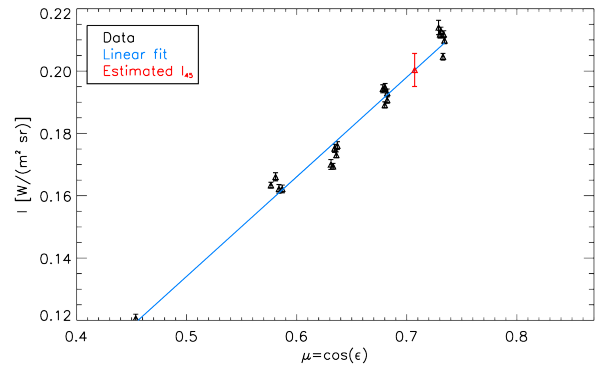
Fig. 4. JIRAM data from a given location acquired at different emission angles are used to infer, by interpolation of a linear fit, the value at the reference emission angle of 45^\circ . Panels a.-d. present four examples at different absolute signal levels.
