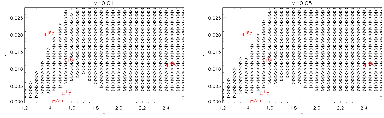
Fig. 11. The plots display with black triangles the regions of the n - k space (real and imaginary parts of refractive index respectively) that satisfy the two constraints 0.85 < \omega_0 < 0.95 and 0.22 < g < 0.52 for any r_{\text{eff}} in the range 0.3 - 3.0 \mu\text{m} . Red squares provide, for reference, the refractive indices at 4.8 \mu\text{m} for different putative components of Jupiter's clouds. Hy : \text{N}_2\text{H}_4 , from Clapp and Miller, Am : \text{NH}_3 , from Howett et al., Fe : \text{NH}_4\text{SH} , from Ferraro et al., Ho : \text{NH}_4\text{SH} , from Howett et al., To : tholin type 2 from Imanaka et al. a. For a size distribution variance of 0.01 b. for a size distribution variance of 0.05 .
