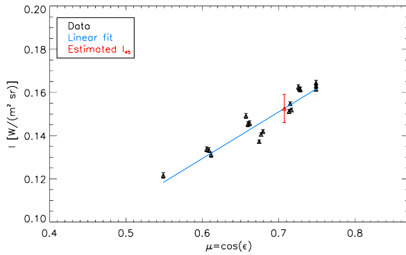
Fig. 4. JIRAM data from a given location acquired at different emission angles are used to infer, by interpolation of a linear fit, the value at the reference emission angle of 45^\circ . Panels a.-d. present four examples at different absolute signal levels.
