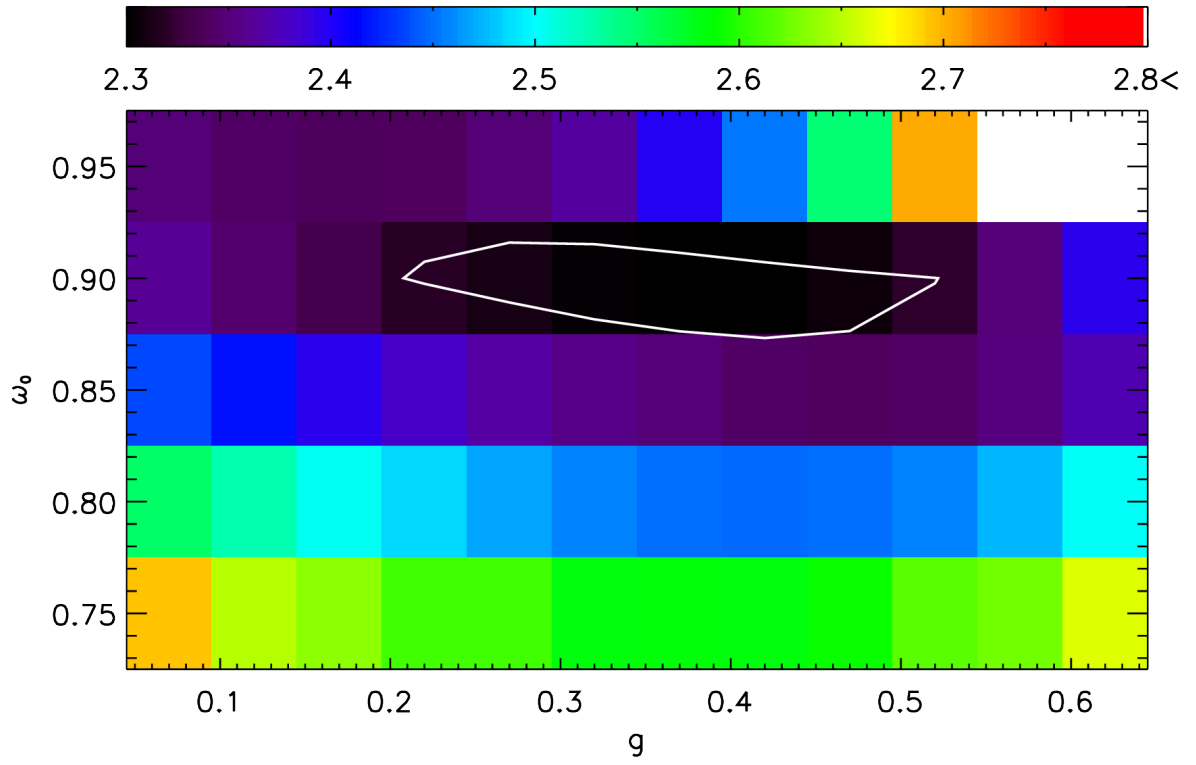
Fig. 8. The dimensionless cost function C – measuring the discrepancy between the observed and theoretical f_0 surfaces (see text for definition) - for different values of \omega_0 and g . The white level curve indicates the 3\sigma uncertainty in the determination of minimum.
