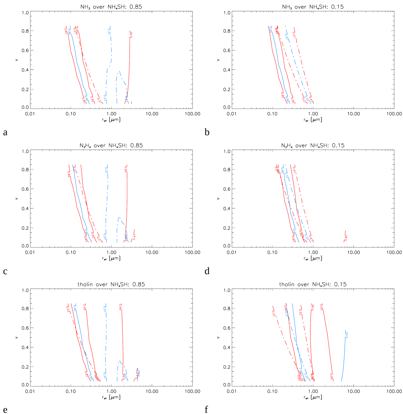
Fig. 12. As fig. 10, for coated particles formed by a \text{NH}_4\text{SH} core (Howett et al.) and different coatings. a.-b. \text{NH}_3 coating. c.-d. \text{N}_2\text{H}_4 coating e.-f. tholin coating. 0.85 and 0.15 labels provide the core-to-particle radii ratio (0.85 large core, 0.15 small core)
