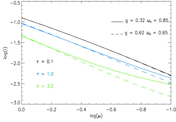
Fig. 2 Examples of theoretical limb darkening functions for typical Hot-Spot conditions, for different cloud opacities \tau . \mu is the cosine of emission angle \epsilon . Note that both axes are in logarithmic form, to highlight deviations from the Minnaret's formulation (see text).
