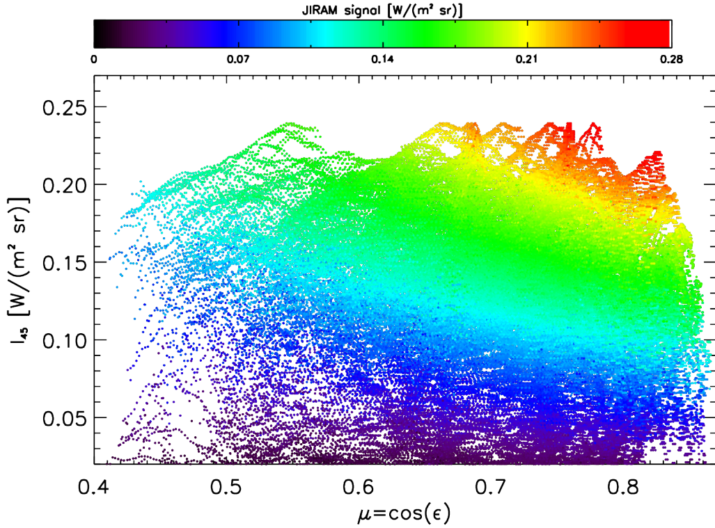
Fig. 6. Experimental sampling of the surface I = f_0(I_{45}, \mu) , as derived from JIRAM observations. Individual points represent individual triplets, as described in the text.
