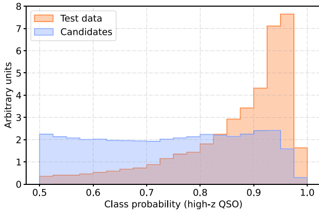
Figure 14. Class probability (high- z QSO) of QSO candidates in the testing data set and in the candidate list, obtained with the PRF trained on colour data. The light blue histogram shows the probability distribution of high- z QSO candidates, while the orange one the high- z class probability distribution of the testing set. A class-probability lower than 0.5 implies that a source is classified as low- z QSO, and as such is not shown in this plot. Both histograms have been normalized so that the integral over the range is equal to one.
