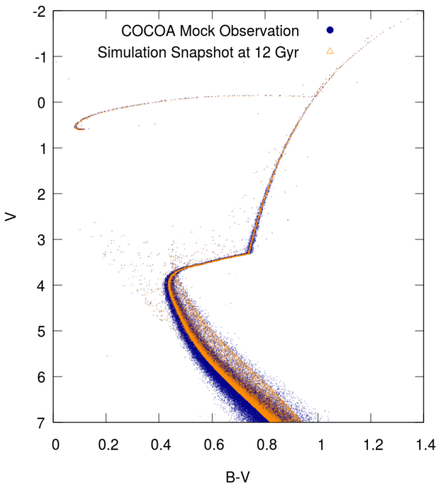
Figure 3. Colour Magnitude Diagram (CMD) for the cluster model at 12 Gyrs. The magnitudes from observations have been scaled to absolute magnitudes by comparing it with the CMD taken from the simulation snapshot. The B-V colour is on the x-axis and the V-band magnitude is on the y-axis. The blue points indicate observed stars from our PSF photometry pipeline. The orange points are from the CMD directly taken from the snapshot of our simulation results.
