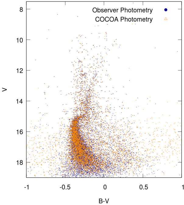
Figure 4. Colour magnitude diagram for an actual observation of the Galactic GC NGC 2808. The magnitudes are instrumental and the orange points show the results from the module in COCOA while the blue points are the photometry results done by observers.
