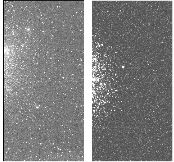
Figure 5. Left: Observational image of the Galactic GC NGC 2808. The observation was carried out in the V/89 filter of the ESO Wide Field Imager (WFI) that is mounted on the 2.2 meter telescope in La Silla, Chile (Dalessandro et al. 2011). Right: Synthetic observational image created using COCOA of a GC model with observational properties comparable to NGC 2808. The parameters for creating this mock observational image were set to replicate the properties of the WFI instrument mounted on a 2.2 meter telescope.
