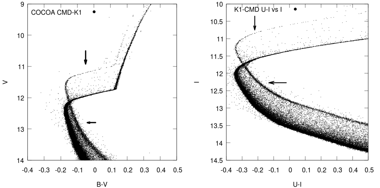
Figure 9. Left Panel: B-V vs V CMD for the K1 model produced using instrumental B and V band magnitudes. There is a prominent second MS due to many binaries with q close to unity that is indicated with the black arrows. Right Panel: U-I vs I CMD for the K1 model. The figure zooms in on part of the CMD close to the MS turn-off. The presence of a large number of binaries (with q close to 1) causes a second sequence which has its own turnoff 3/4 of a magnitude above the turn-off for single stars.
