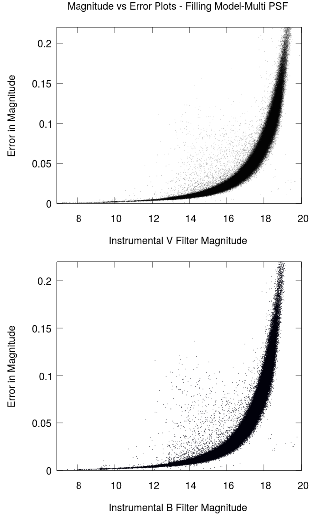
Figure 2. Error vs magnitude plot for V-band and B-band photometry. The x-axis represents the instrumental magnitude and the y-axis represents the error in magnitude.
