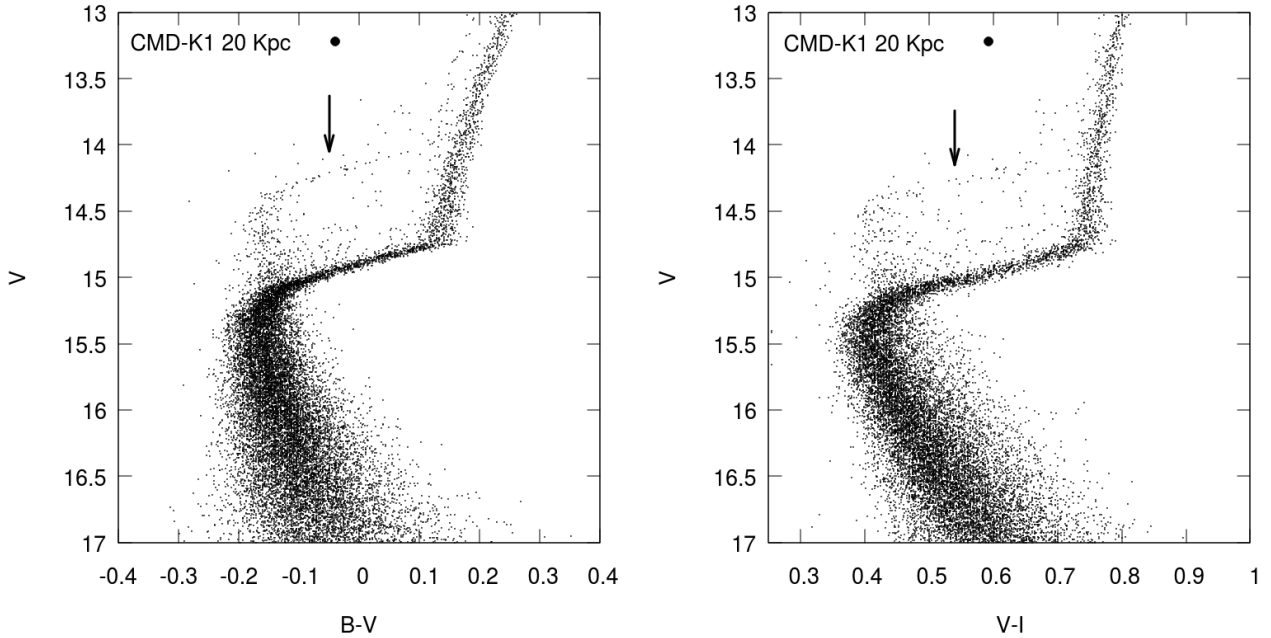
Figure 11. Left Panel: B-V vs V CMD for the K1 model. The cluster was projected at a distance of 20 kpc and the spatial resolution of the instrument was 0.08 arcsec/pixel. The second sequence due to binaries with nearly equal mass components is visible above the MS turn-off and is indicated with the black arrow. Right Panel: V-I vs V CMD for the K1 model using instrumental V and I band magnitudes. The second sequence above the MS turn-off is indicated with the black arrow.
