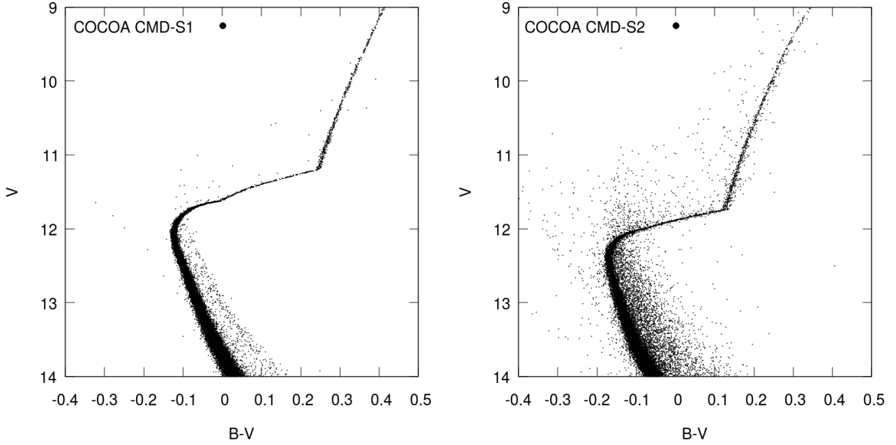
Figure 10. Left Panel: B-V vs V CMD for the S1 model. Even though this model is initially sparse, no second sequence due to equal mass ratio binaries is seen. CMDs produced using other filters also showed an absence of the second sequence. Right Panel: B-V vs V CMD for the S2 model. Similar to model S1, there is no presence of a prominent second sequence due to equal mass binaries that was seen in models K1 and K2.
