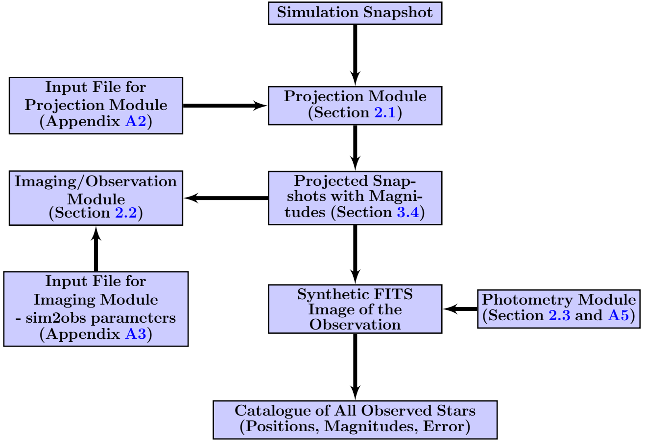
Figure 1. COCOA Flow Chart: A schematic diagram of the main steps and the sequence of the code.
