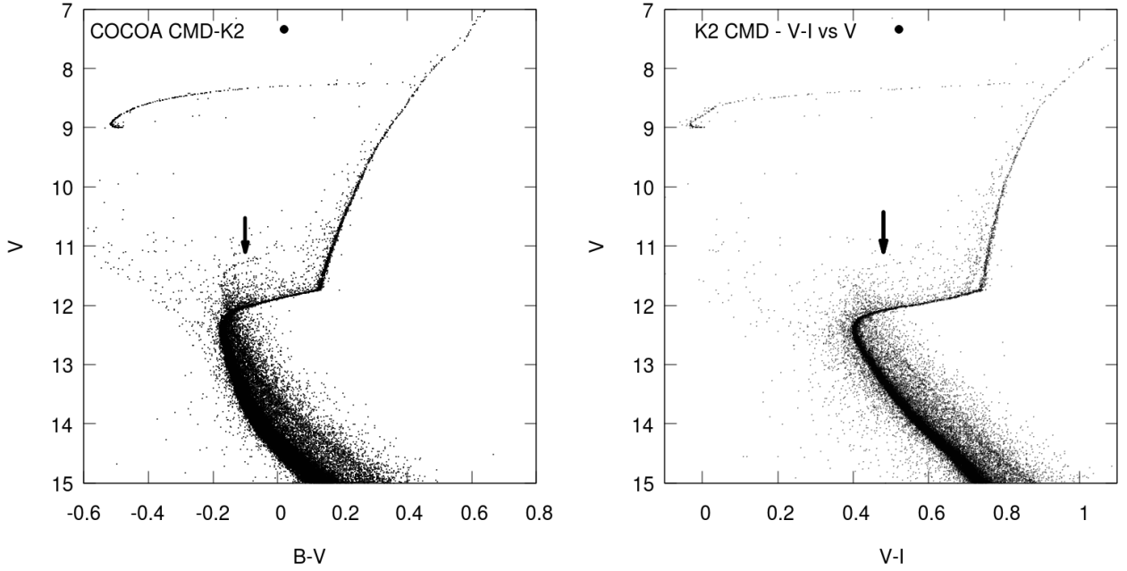
Figure 8. Left Panel: Shows the B-V vs V CMD for the K2 model using instrumental B and V band magnitudes. There are indications of the presence of a second main sequence due to many binaries with q (mass ratio) close to unity. The black arrows shows these binaries that are visible above the MS turn-off. Right Panel: Shows the V-I vs V CMD for the same model which is significantly denser than the K1 model. Due to this higher density and overall lower binary fraction, the photometric errors are larger and it becomes difficult to distinguish the second sequence. Also with higher density, a significant number of such binaries are disrupted. However, there are still binaries with nearly equal mass components above the MS turn-off that are indicated with the black arrow.
