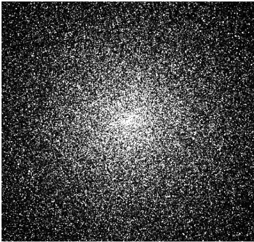
Figure 7. I-band image of the innermost frame imaging the core of the cluster model K2. 2048 \times 2048 pixels. The cluster was imaged with a high spatial resolution telescope with pixel scale of 0.08 arcsec/pixel. The projected distance to cluster model was 5 kpc.
