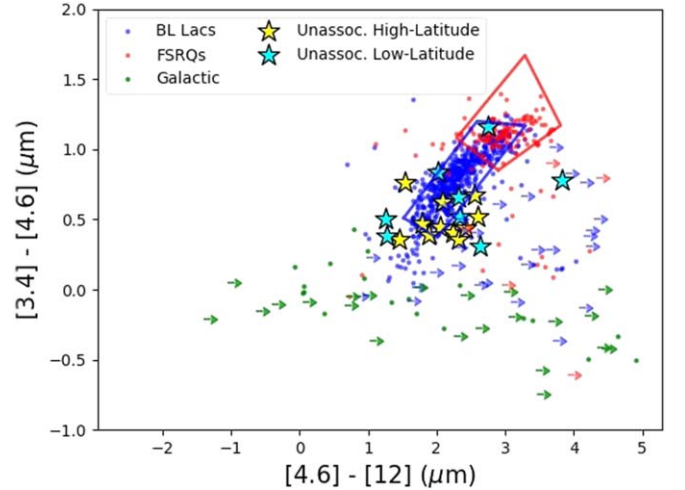
Figure 3. The WISE blazar strip in the color space w1 (3.4 \mu\text{m} ) – w2 (4.6 \mu\text{m} ) vs. w2 - w3 (12 \mu\text{m} ). The blue and red circles represent 439 known BL Lac objects and FSRQs used in our machine-learning algorithm while known Galactic sources are in green. The coordinates for the strip can be found in Massaro et al. (2012). The arrows represent sources with only an upper limit on the w3 magnitude. Two Galactic sources with a w1 - w2 value < -1 are not shown to improve readability.
