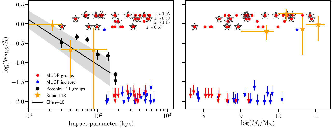
Figure 10. Rest-frame equivalent width ( W ) for the \text{Mg II } \lambda 2796 \text{ \AA} absorption line as a function of impact parameter (projected distance of each galaxy from the QSO-SE sightline for MUDF galaxies, left-hand panel) and of the galaxy stellar mass (right-hand panel). Galaxies in the MUDF footprint are shown as red circles if they reside in a group and as blue circles if they are isolated. The arrows (red for galaxies in groups and blue for isolated galaxies) show 2\sigma upper limits measured on the UVES spectrum in a 10 \text{ km s}^{-1} velocity window centred at the redshift of each galaxy. The black empty stars show galaxies which have a redshift within the \text{Mg II} absorption profile for the strong absorbers shown in Fig. 9. The redshift of the groups are shown in the left-hand panel at the y-axis levels of the corresponding values of W . The black line is the best-fitting relation (with the 1\sigma confidence area shaded in grey) between W and impact parameter from Chen et al. (2010). The orange stars and black circles are obtained from stacking galaxy–galaxy pairs from the sample of isolated galaxies of Rubin et al. (2018a) and the sample of group galaxies of Bordoloi et al. (2011).
