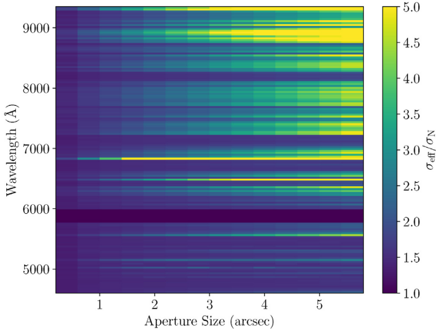
Figure 3. Ratio between the flux dispersion in apertures of varying size ( \sigma_{\text{eff}} ) and the error derived propagating the variance ( \sigma_N ), as computed across the MUDF datacube in a 5 \text{ \AA} window (4 pixels) as a function of wavelength and aperture size. The dark stripe just below 6000 \text{ \AA} is the region without valid data due to the scattered light from the AO laser.
