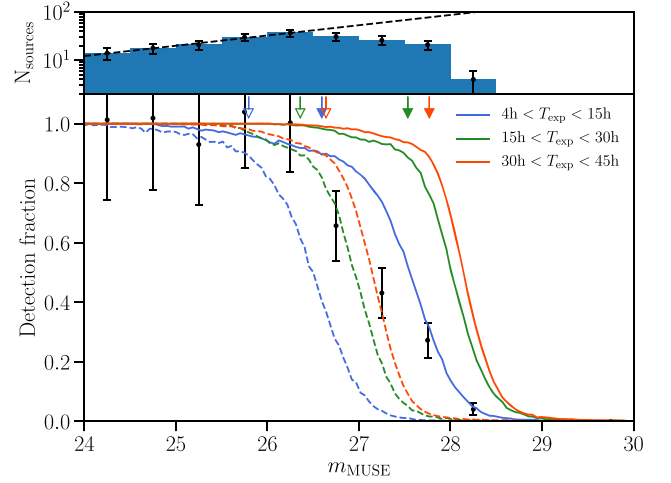
Figure 6. Top panel: Number of galaxies extracted as a function of the magnitude in the detection image. The grey dashed line shows the expected number of galaxies determined from a linear fit to the region between m_{\text{MUSE}} > 24 \text{ mag} and m_{\text{MUSE}} < 26.5 \text{ mag} . Bottom panel: Fraction of mock sources detected by SEXTRACTOR. The solid lines are for the injection of Gaussian sources with a FWHM of 0.6 arcsec. The dashed lines are for sources with an exponential profile with scale-length equal to 0.26 arcsec and PSF convolved. Lines of different colours are for different exposure times in the MUDF map. The arrows (filled for point sources and empty for extended ones) mark the faintest magnitude at which we are 90 per cent complete in each bin of exposure time. The black points (with error bars) show the empirical detection fraction determined as the ratio of the detected galaxies relative to the expected number from the linear fit in the top panel.
