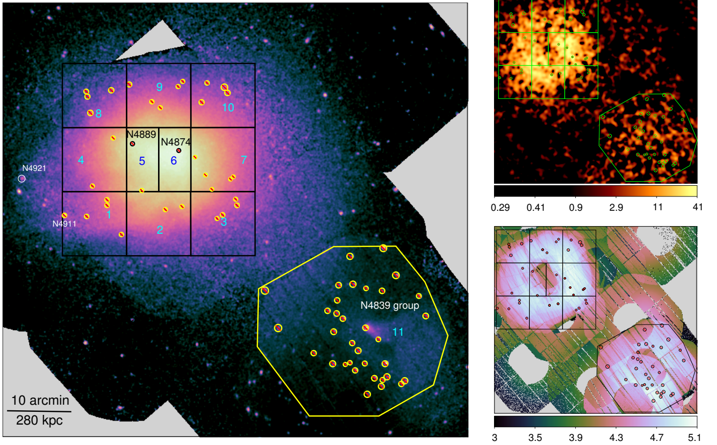
Fig. 19. Regions examined in Coma. ( Left panel ) The regions plotted on an exposure-corrected surface brightness image in the 0.5 to 2.0 keV band. ( Top-right panel ) Image in the Fe-K band, after subtracting continuum, in 10^{-3} counts per 1.6 arcsec pixel. ( Bottom-right panel ) Fe-K exposure map in log s, including the effect of vignetting and the Cu hole.
