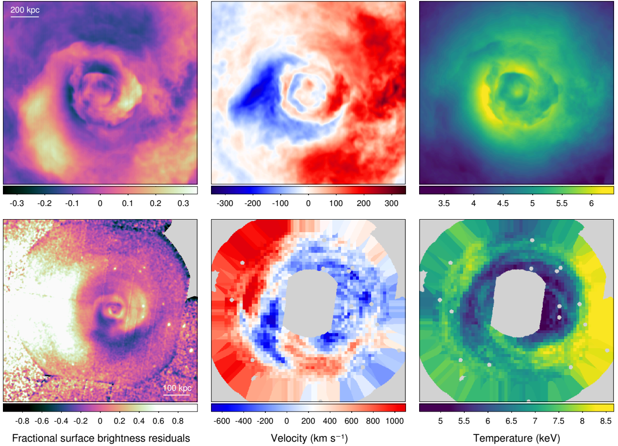
Fig. 18. Comparison of a sloshing simulation ( top row ) and data for the Perseus cluster (Fig. 16; bottom row ). The columns show surface brightness residuals ( left ), velocity ( centre ) and temperature ( right ). The simulation is of a Perseus-like cluster which has bulk sloshing motions and turbulence initiated by an off-centre encounter with a subcluster of 1/5 its mass, from ZuHone et al. (2010, 2018).
