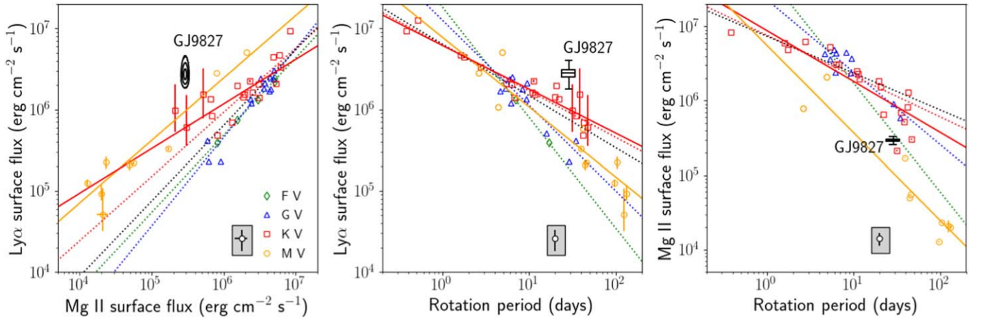
Figure 5. GJ 9827’s Ly \alpha and Mg II surface fluxes (corrected for ISM absorption) and rotation period are compared to other F, G, K, and M stars from the literature (Wood et al. 2005; Youngblood et al. 2016). The literature sample is shown by colored open symbols with corresponding best-fit linear regressions (dashed lines: from Wood et al. 2005; solid lines: from Youngblood et al. 2016). The example error bars in each panel apply to colored symbols without error bars. In the left panel, the 68%, 95%, and 99.7% confidence intervals from our simultaneous Ly \alpha and Mg II reconstruction are shown as black contours. In the right two panels, the black box and whisker symbol shows the median Ly \alpha and Mg II surface flux with the 68% and 95% confidence intervals as the box and whiskers, respectively, at the assumed stellar rotation period (28.72 days; Rice et al. 2019).
