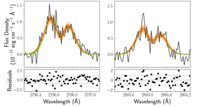
Figure 4. Reconstructed (orange dashed line) and fitted (attenuated; solid green line) Mg II profiles are shown. The ISM absorption is weak and centered at 2796.38 and 2803.56 Å; the effect on the resultant profile is small. In the left panel, the dotted green line shows the model of the attenuated profile with the 2\sigma upper limit on the Mg II column density ( \log_{10}N(\text{Mg II}) < 13.33 ). The bottom panels show the residuals (data-model)/(data uncertainty).
