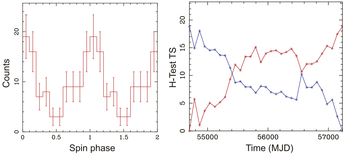
Figure 4. Left: gamma-ray pulse profile of AE Aqr in the 1.7–10 GeV energy range, with a ROI radius of 0.6^\circ folded on our timing ephemeris. Two full rotations are shown for clarity. Right: H-test TS value of AE Aqr as a function of time. The red line represents the trend of the TS value as data is accumulating from the start of the mission, while the blue line represents the same trend as data is accumulating from the end of the integration.
