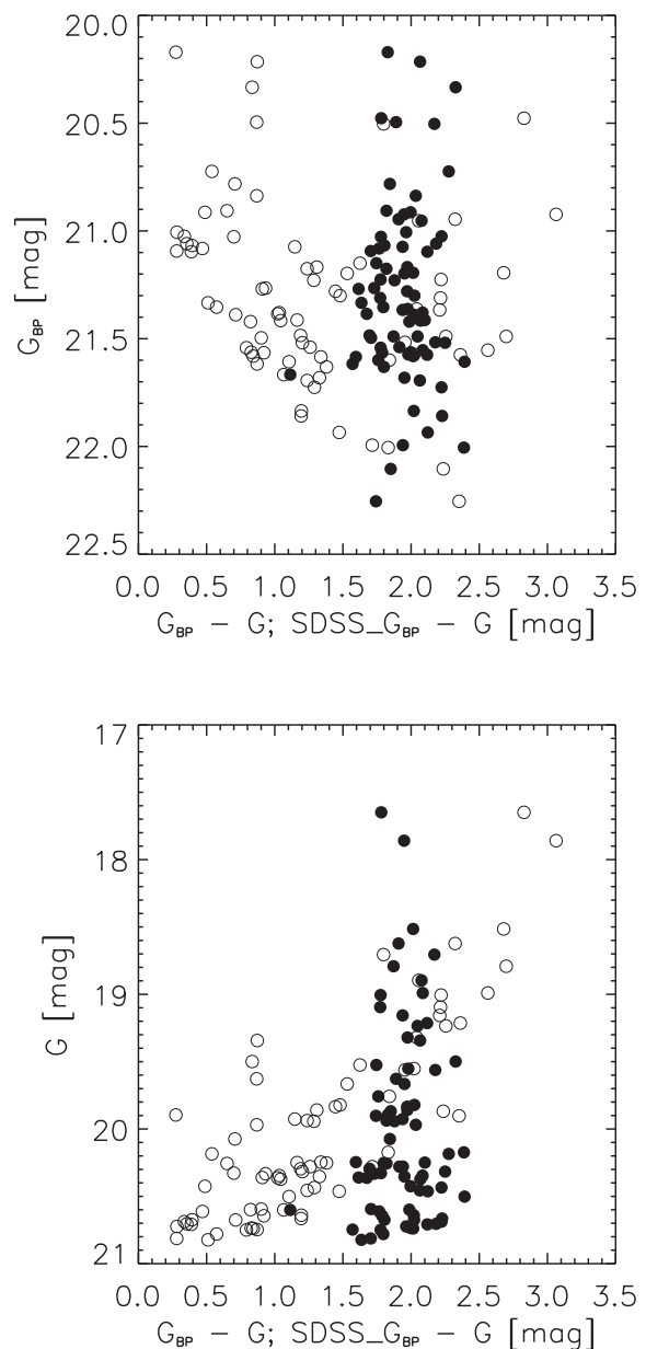
Figure 7. Top: zoom on the objects with SDSS magnitudes from Fig. 5. Open circles as before using G_{BP} versus G_{BP} - G ; filled circles are the same objects however plotting G_{BP} versus SDSSG_{BP} - G . Bottom: same as top panel figure but plotting G instead of G_{BP} on the ordinate.
