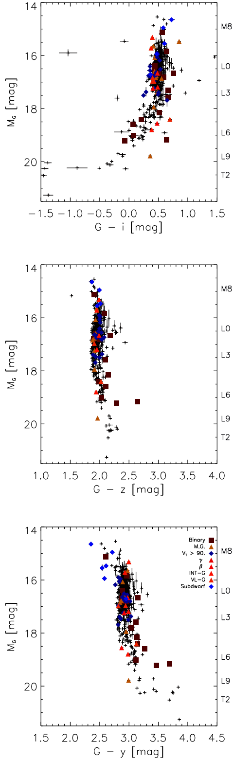
Figure 9. Colour-magnitude diagrams. G -band absolute magnitude as a function of G - i , G - z , and G - y from the Pan-STARRS PS1. The legend in the third panel indicates the symbols used for spectral type qualifications, binarity, and high tangential velocity objects.
