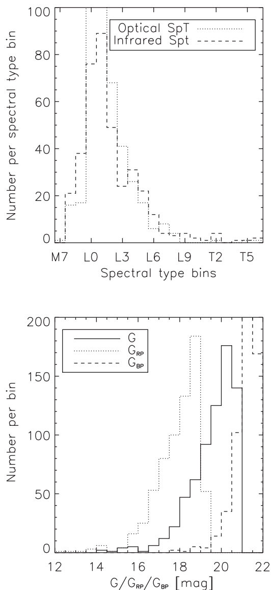
Figure 1. Top: distribution of optical and infrared spectral types in the GUCDSat. Optical L0 and L1 bins have been truncated (they contain 202 and 105 objects, respectively). Bottom: distribution of Gaia magnitudes in the GUCDSat.
