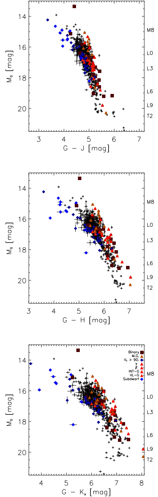
Figure 10. Same as Fig. 9 but for G - J , G - H , and G - K_s colours from the 2MASS PSC.
