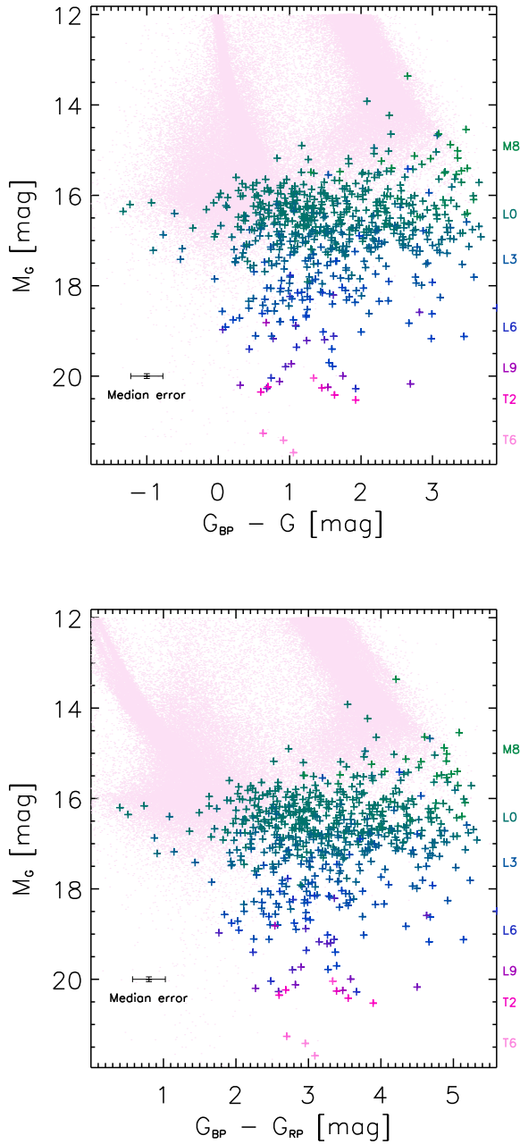
Figure 4. Colour-magnitude diagrams for absolute G versus G_{BP} - G (top) and G_{BP} - G_{RP} (bottom). The light pink points are all objects within 100 pc, the crosses are the GUCDScat entries colour coded by spectral type as indicated on the right hand side. Plotted in the lower left are error bars that are equivalent to the median uncertainty.
