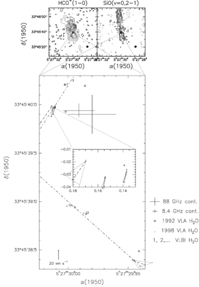
Figure 1. The upper panels show the contour maps of the OVRO high-velocity molecular line emission for \text{HCO}^+(1 \rightarrow 0) (left) and \text{SiO}(v = 0, 2 \rightarrow 1) (right). The area at the center of the OVRO field of view, where the 22.2 GHz water emission has been detected by our VLBI observations, is expanded in the lower panel. This shows the spatial distribution of the VLBI features superimposed on top of the distribution of the VLA emission centers. The arrows indicate the measured proper motions, with dashed lines used in case of more uncertain values. The dotted triangles drawn around the proper motion vectors represent the amplitude and orientation uncertainty. The region in the northeast corner enclosed by the dotted lines is shown in greater detail in the box at the center of the lower panel, whose coordinates are arcsec offsets relative to the position: \text{RA} = 05^{\text{h}}27^{\text{m}}30^{\text{s}} ; \text{DEC} = +33^{\circ}45'40'' . The amplitude scale for the proper motions is given at the bottom left corner of the panel. For each of the two Groups of VLBI maser features, the dot-dashed line indicates the axis whose average distance from the feature positions is minimum.
