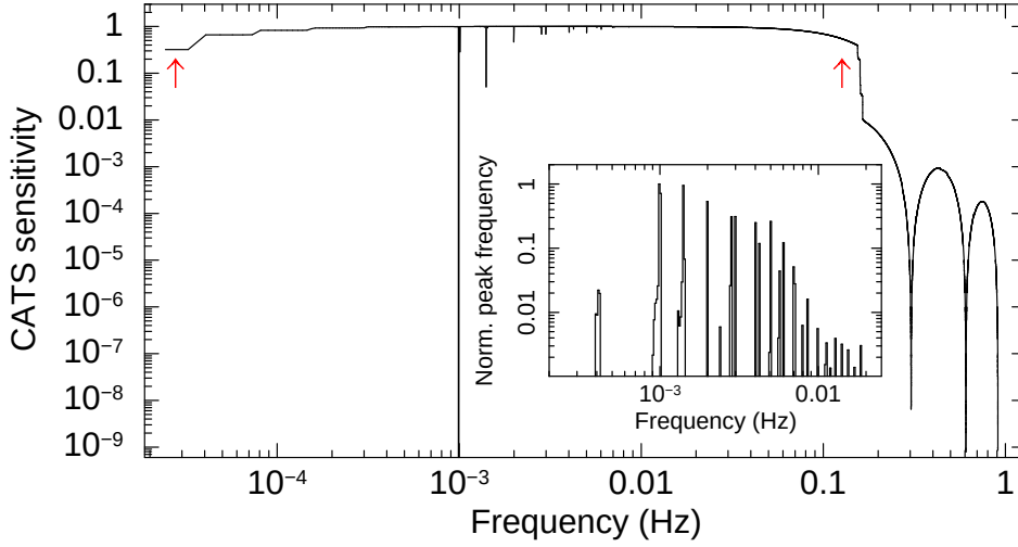
Figure 4. Sensitivity map as a function of frequency for the CATS signal search: drops in the sensitivity are due to the dithering signals (in the 10^{-3} – 10^{-2} Hz interval) and the sampling times (above 0.1 Hz; see Section 5 for details). The red arrows mark the longest and shortest period discovered by the CATS pipeline. In the inset we show the more frequent spurious signals detected by the pipeline during the search, the most prominent being at the dithering frequencies plus many harmonics.
