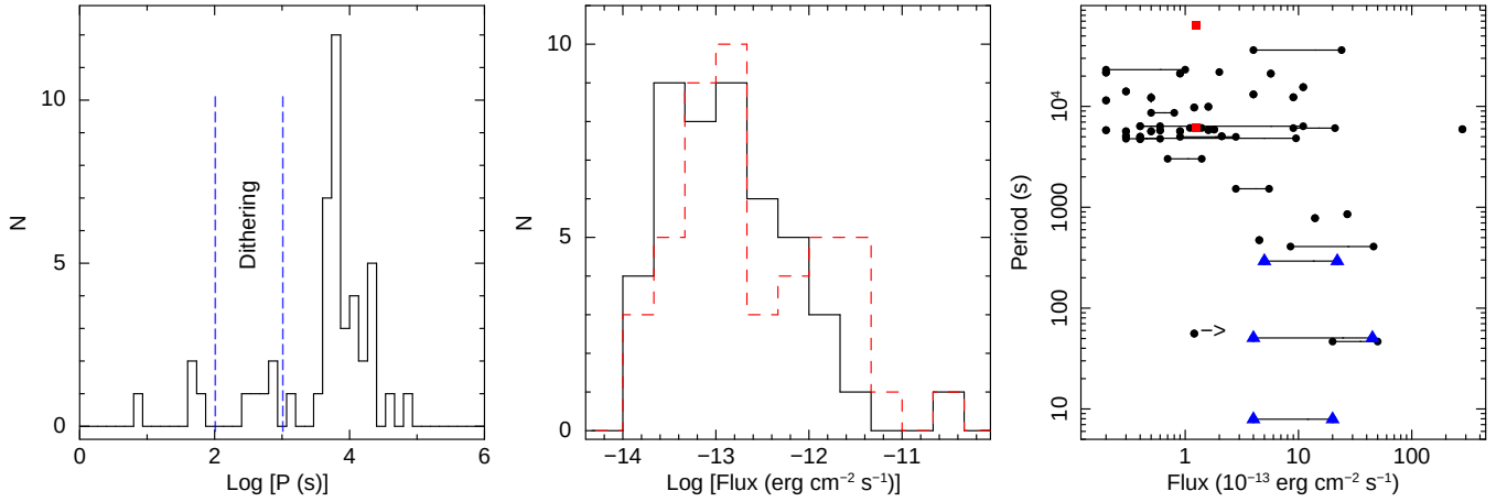
Figure 5. Main properties of the CATS@BAR sample of new X-ray pulsators. From left to the right are shown the period distribution (left panel), the flux distribution (central panel), and the period versus flux plane (right panel), where the solid lines mark the objects detected at different flux levels (the right arrow marks a variable object for which we can rely upon only one dataset), the (blue) triangles corresponds to the transient NSs in the Be X-ray binaries of the SMC, and the (red) squares the spin and orbital periods of the new CV/IP in the field of view of the Circinus galaxy. In the left panel we marked the period interval where the effects of the spacecraft dithering hampers the detection of true signals. In the central panel the solid black and the stepped red lines correspond to the flux distributions obtained by assuming the minimum and maximum fluxes of variable objects, respectively.
