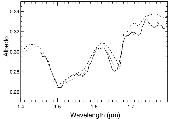
Fig. 2. Spectrum zoom of (50000) Quaoar (Q1, solid line) and corresponding best-fitting spectral model (dotted line, described in Table 3) and equivalent model calculated with pure CH 4 alone (dashed line).
